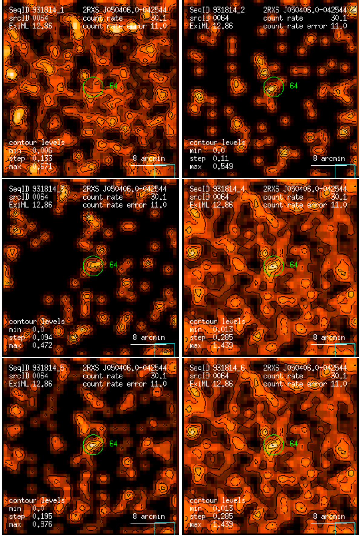
Figure 64: RASS 931814: detection 0064: band rate images, Gaussian filter: (1) PSPC channels 11 – 41, (2) 52 – 90, (3) 91 – 201, (4) 11 – 235, (5) 52 – 201, (6) 11 – 201. Broad band rates in counts/ks. Band rate contour levels in counts/ks/arcmin 2 .
