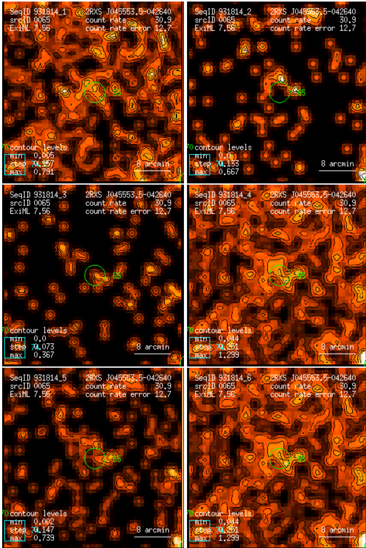
Figure 65: RASS 931814: detection 0065: band rate images, Gaussian filter: (1) PSPC channels 11 – 41, (2) 52 – 90, (3) 91 – 201, (4) 11 – 235, (5) 52 – 201, (6) 11 – 201. Broad band rates in counts/ks. Band rate contour levels in counts/ks/arcmin 2 .
