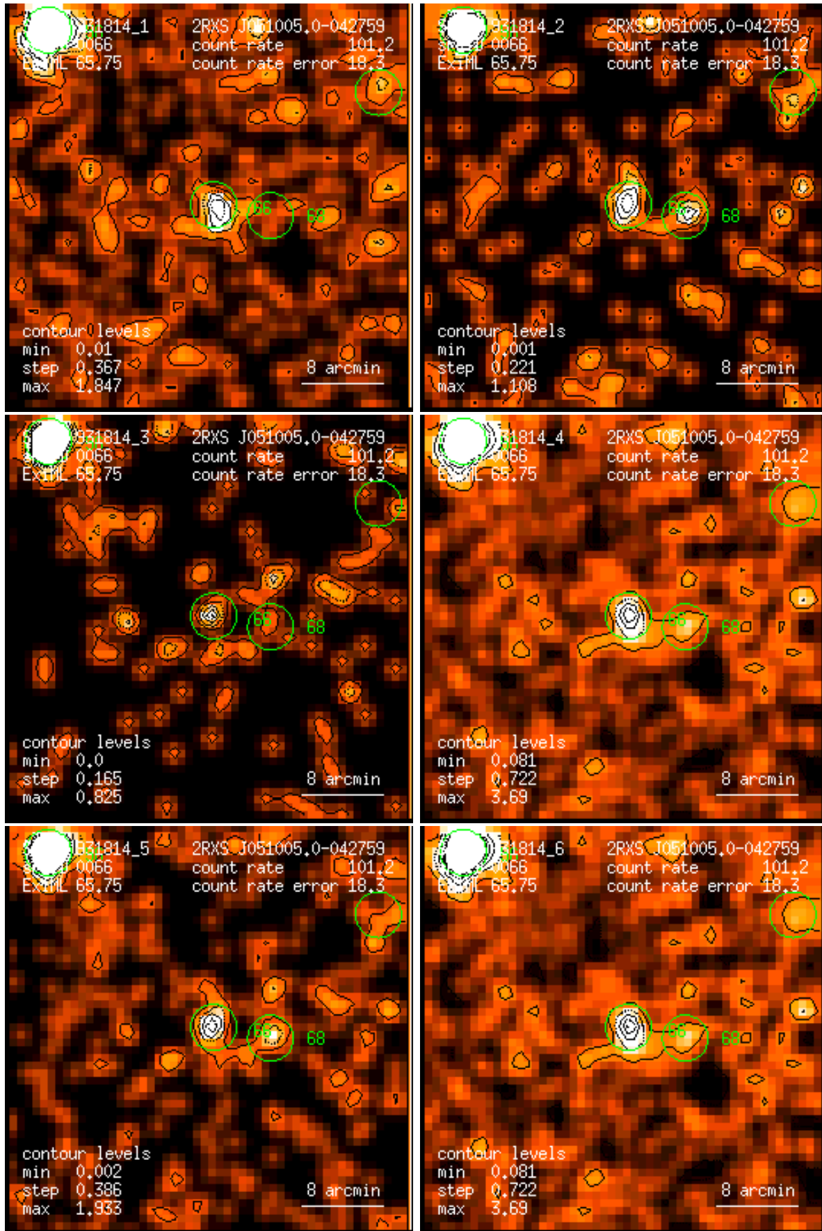
Figure 66: RASS 931814: detection 0066: band rate images, Gaussian filter: (1) PSPC channels 11 – 41, (2) 52 – 90, (3) 91 – 201, (4) 11 – 235, (5) 52 – 201, (6) 11 – 201. Broad band rates in counts/ks. Band rate contour levels in counts/ks/arcmin 2 .
