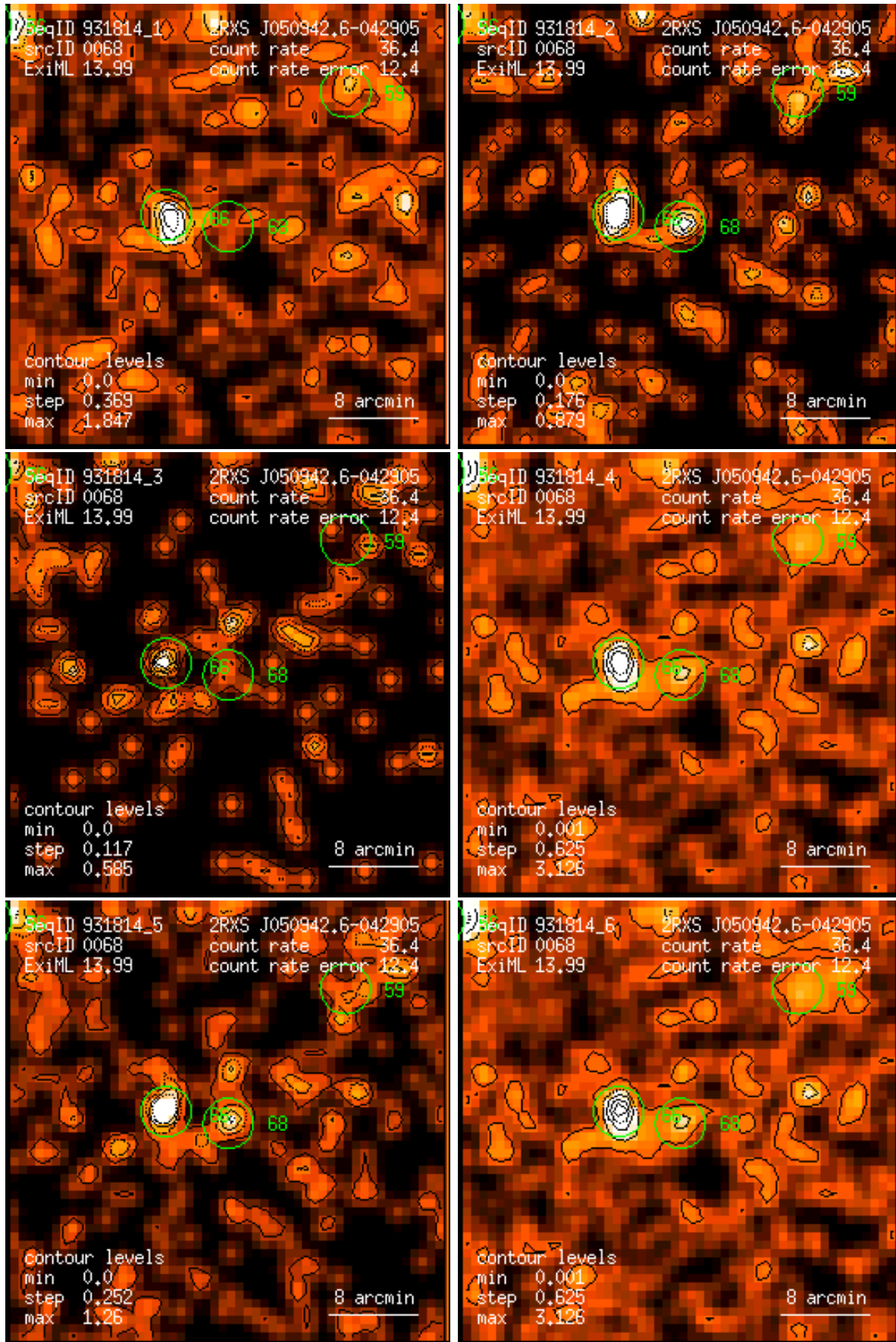
Figure 68: RASS 931814: detection 0068: band rate images, Gaussian filter: (1) PSPC channels 11 – 41, (2) 52 – 90, (3) 91 – 201, (4) 11 – 235, (5) 52 – 201, (6) 11 – 201. Broad band rates in counts/ks. Band rate contour levels in counts/ks/arcmin 2 .
