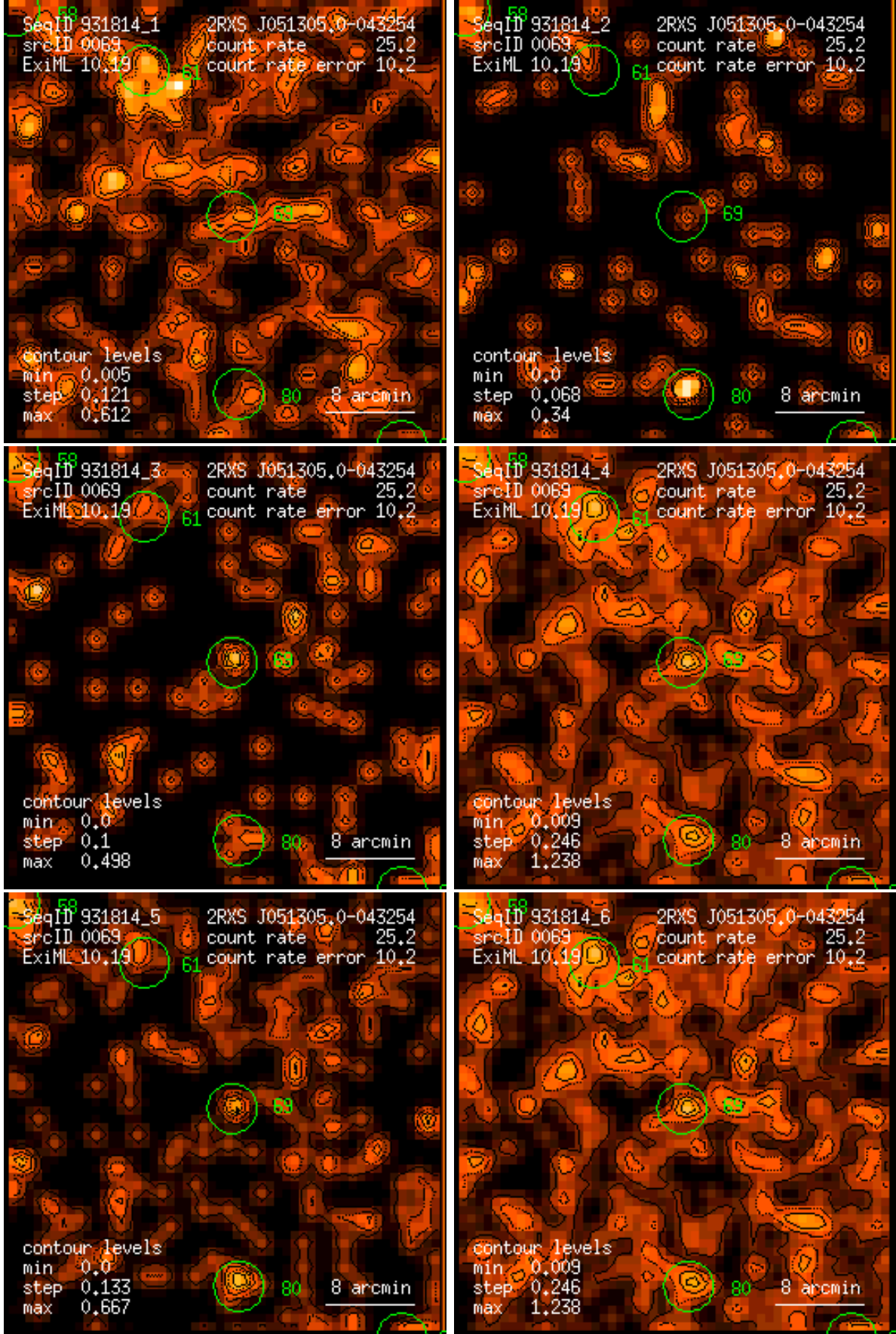
Figure 69: RASS 931814: detection 0069: band rate images, Gaussian filter: (1) PSPC channels 11 – 41, (2) 52 – 90, (3) 91 – 201, (4) 11 – 235, (5) 52 – 201, (6) 11 – 201. Broad band rates in counts/ks. Band rate contour levels in counts/ks/arcmin 2 .
