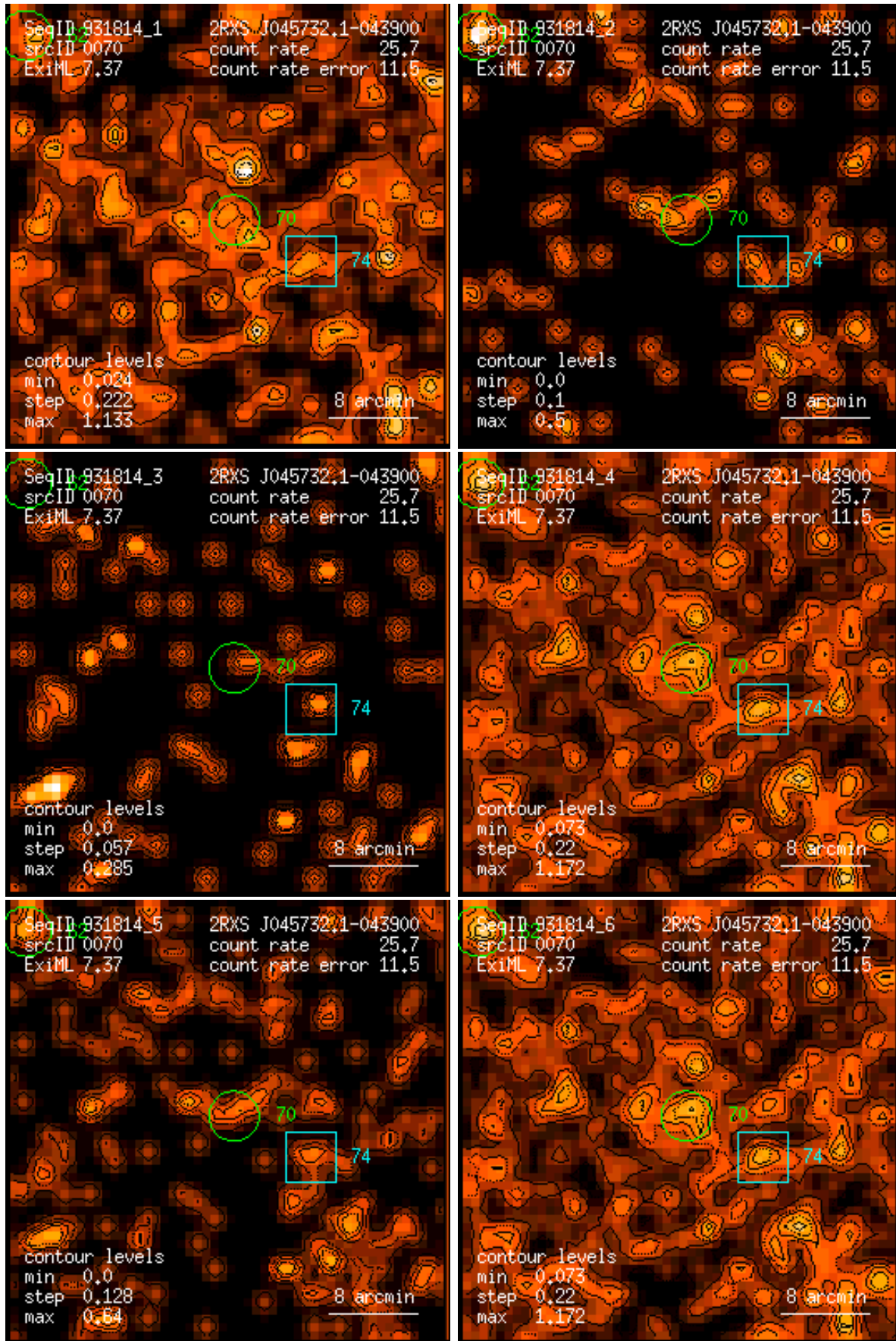
Figure 70: RASS 931814: detection 0070: band rate images, Gaussian filter: (1) PSPC channels 11 – 41, (2) 52 – 90, (3) 91 – 201, (4) 11 – 235, (5) 52 – 201, (6) 11 – 201. Broad band rates in counts/ks. Band rate contour levels in counts/ks/arcmin 2 .
