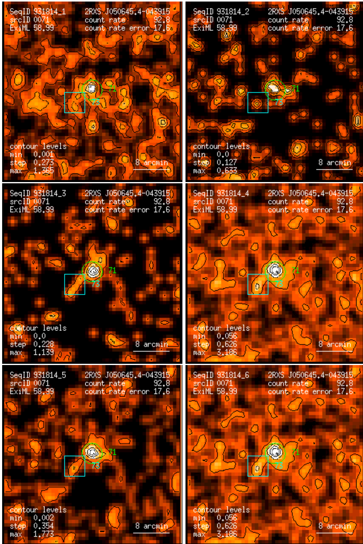
Figure 71: RASS 931814: detection 0071: band rate images, Gaussian filter: (1) PSPC channels 11 – 41, (2) 52 – 90, (3) 91 – 201, (4) 11 – 235, (5) 52 – 201, (6) 11 – 201. Broad band rates in counts/ks. Band rate contour levels in counts/ks/arcmin 2 .
