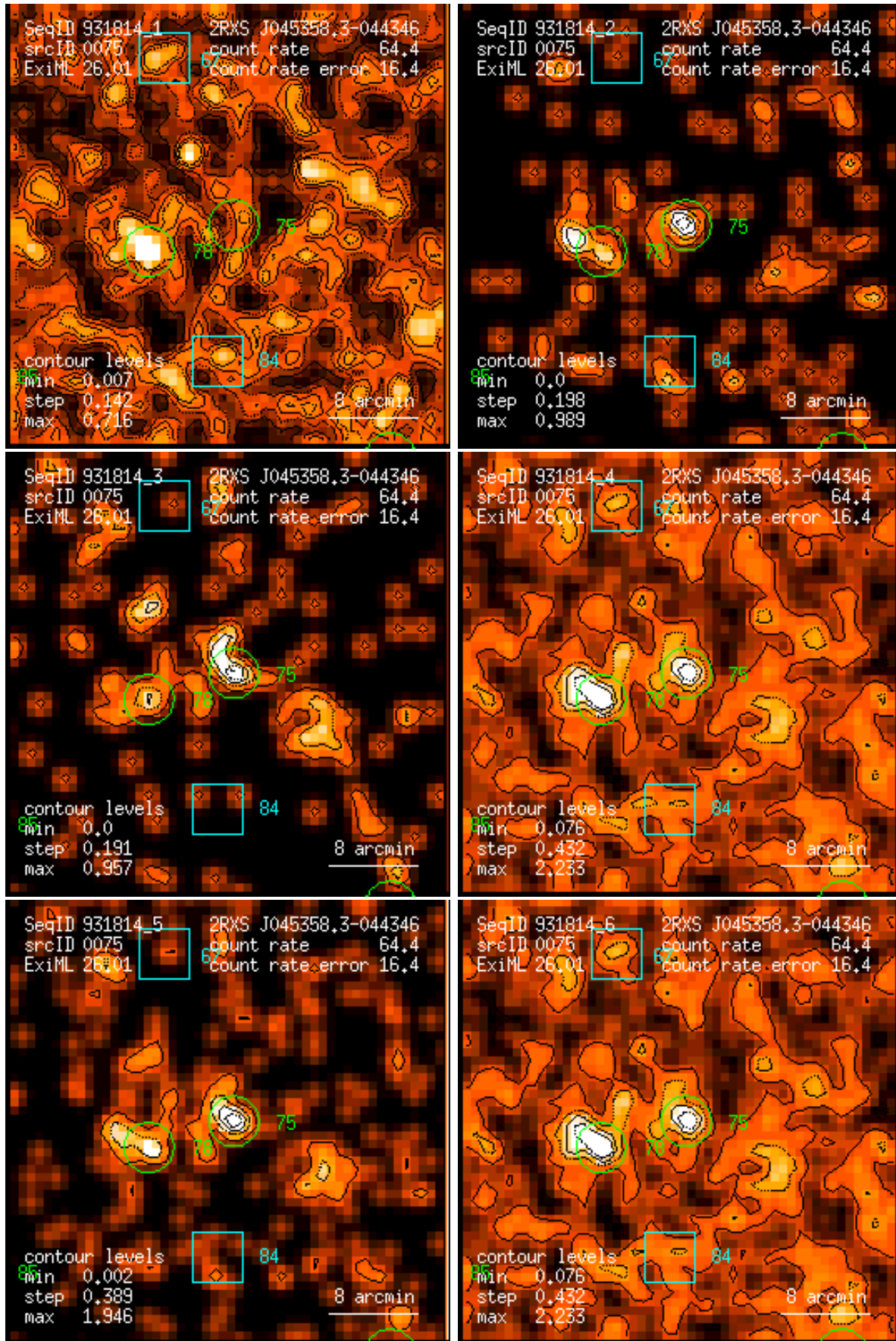
Figure 75: RASS 931814: detection 0075: band rate images, Gaussian filter: (1) PSPC channels 11 – 41, (2) 52 – 90, (3) 91 – 201, (4) 11 – 235, (5) 52 – 201, (6) 11 – 201. Broad band rates in counts/ks. Band rate contour levels in counts/ks/arcmin 2 .
