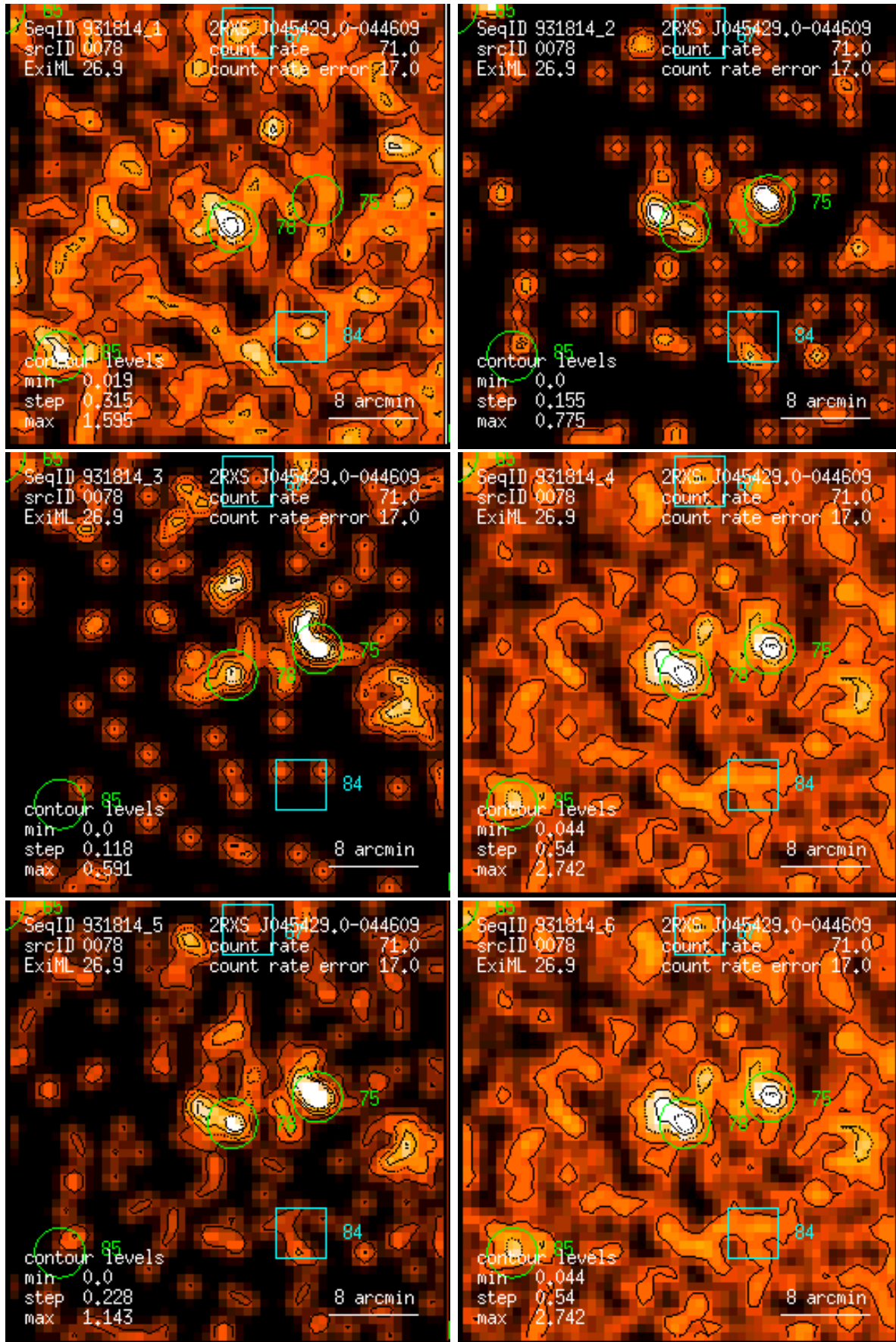
Figure 78: RASS 931814: detection 0078: band rate images, Gaussian filter: (1) PSPC channels 11 – 41, (2) 52 – 90, (3) 91 – 201, (4) 11 – 235, (5) 52 – 201, (6) 11 – 201. Broad band rates in counts/ks. Band rate contour levels in counts/ks/arcmin 2 .
