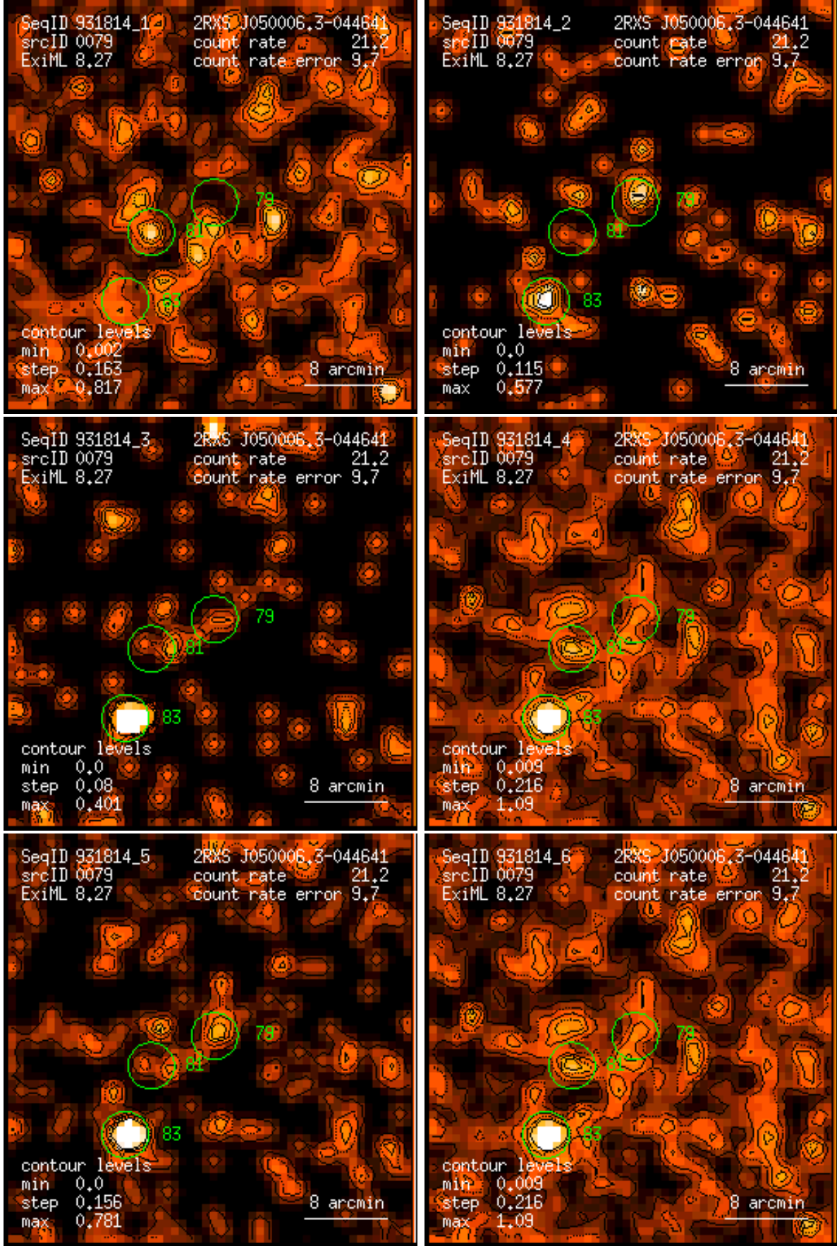
Figure 79: RASS 931814: detection 0079: band rate images, Gaussian filter: (1) PSPC channels 11 – 41, (2) 52 – 90, (3) 91 – 201, (4) 11 – 235, (5) 52 – 201, (6) 11 – 201. Broad band rates in counts/ks. Band rate contour levels in counts/ks/arcmin 2 .
