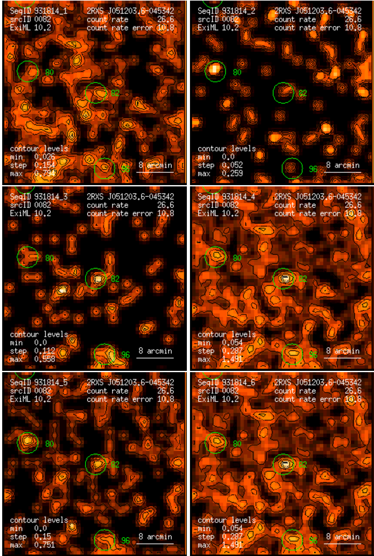
Figure 82: RASS 931814: detection 0082: band rate images, Gaussian filter: (1) PSPC channels 11 – 41, (2) 52 – 90, (3) 91 – 201, (4) 11 – 235, (5) 52 – 201, (6) 11 – 201. Broad band rates in counts/ks. Band rate contour levels in counts/ks/arcmin 2 .
