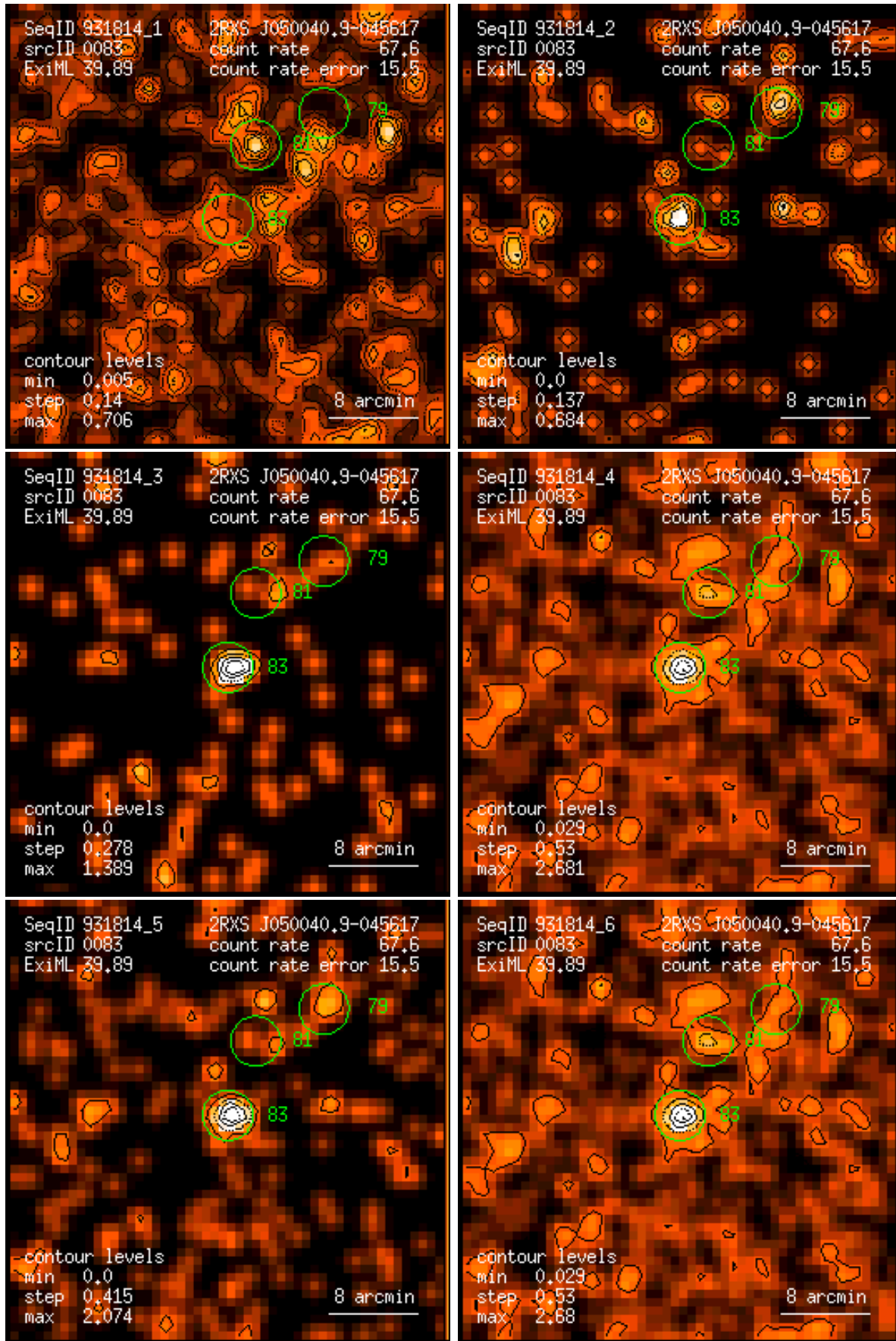
Figure 83: RASS 931814: detection 0083: band rate images, Gaussian filter: (1) PSPC channels 11 – 41, (2) 52 – 90, (3) 91 – 201, (4) 11 – 235, (5) 52 – 201, (6) 11 – 201. Broad band rates in counts/ks. Band rate contour levels in counts/ks/arcmin 2 .
