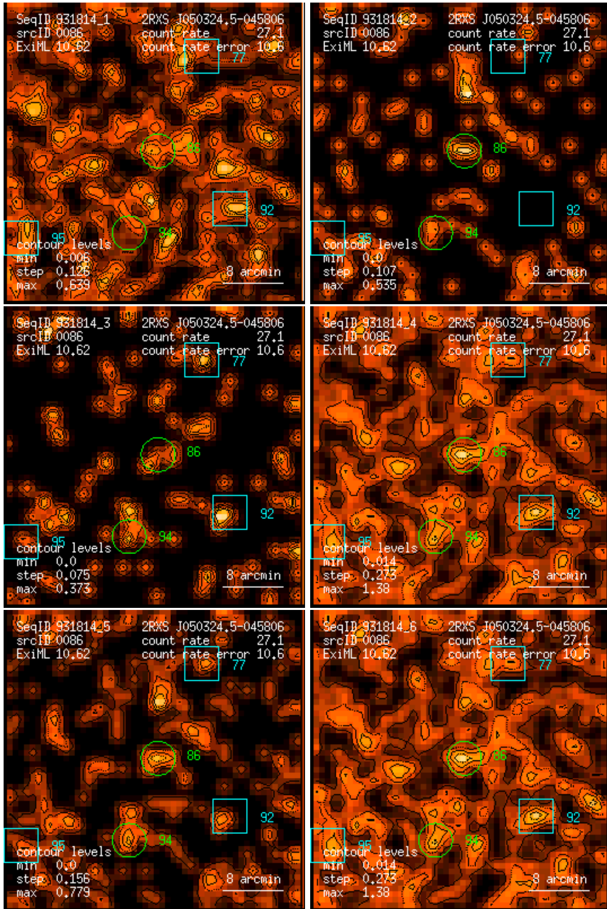
Figure 86: RASS 931814: detection 0086: band rate images, Gaussian filter: (1) PSPC channels 11 – 41, (2) 52 – 90, (3) 91 – 201, (4) 11 – 235, (5) 52 – 201, (6) 11 – 201. Broad band rates in counts/ks. Band rate contour levels in counts/ks/arcmin 2 .
