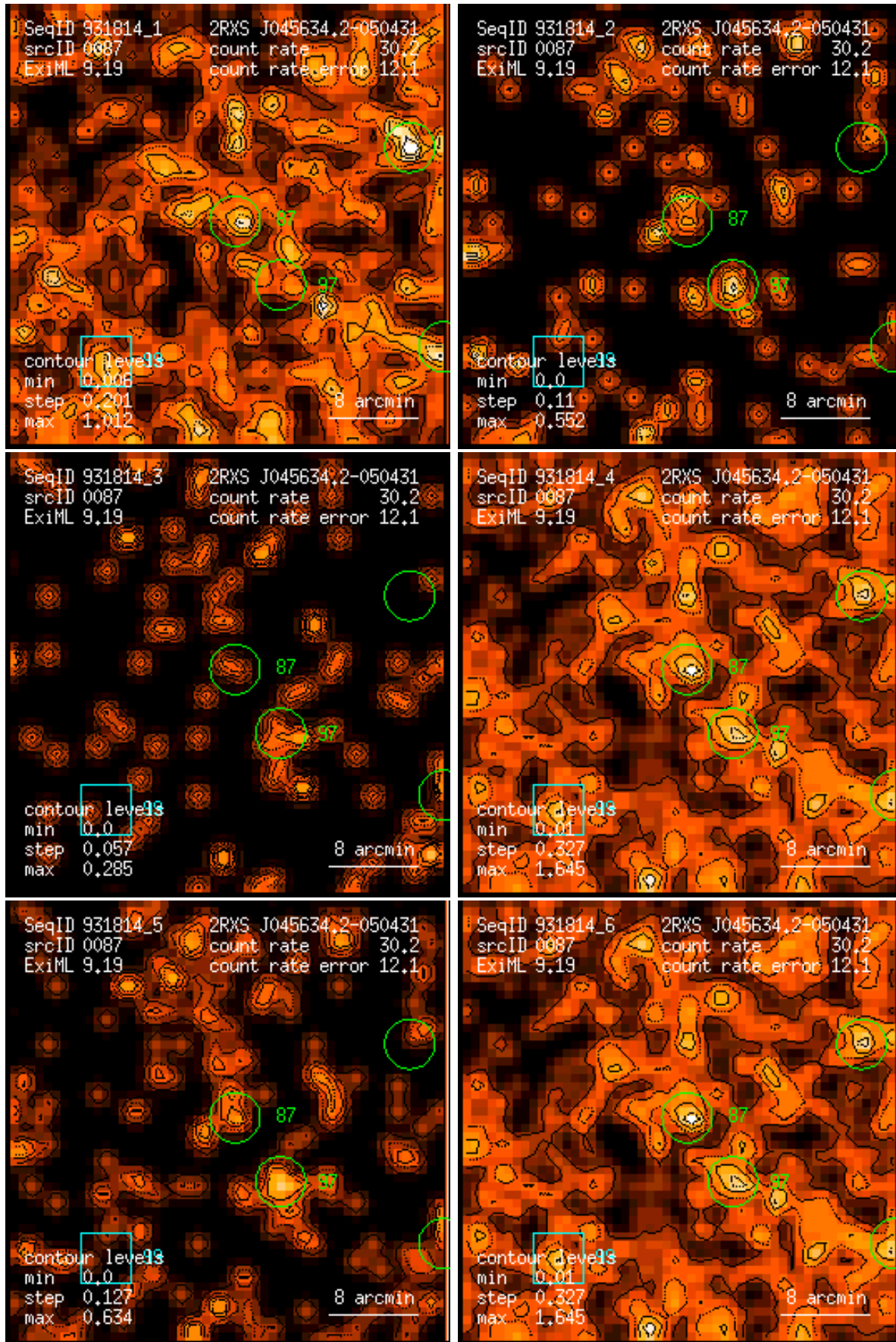
Figure 87: RASS 931814: detection 0087: band rate images, Gaussian filter: (1) PSPC channels 11 – 41, (2) 52 – 90, (3) 91 – 201, (4) 11 – 235, (5) 52 – 201, (6) 11 – 201. Broad band rates in counts/ks. Band rate contour levels in counts/ks/arcmin 2 .
