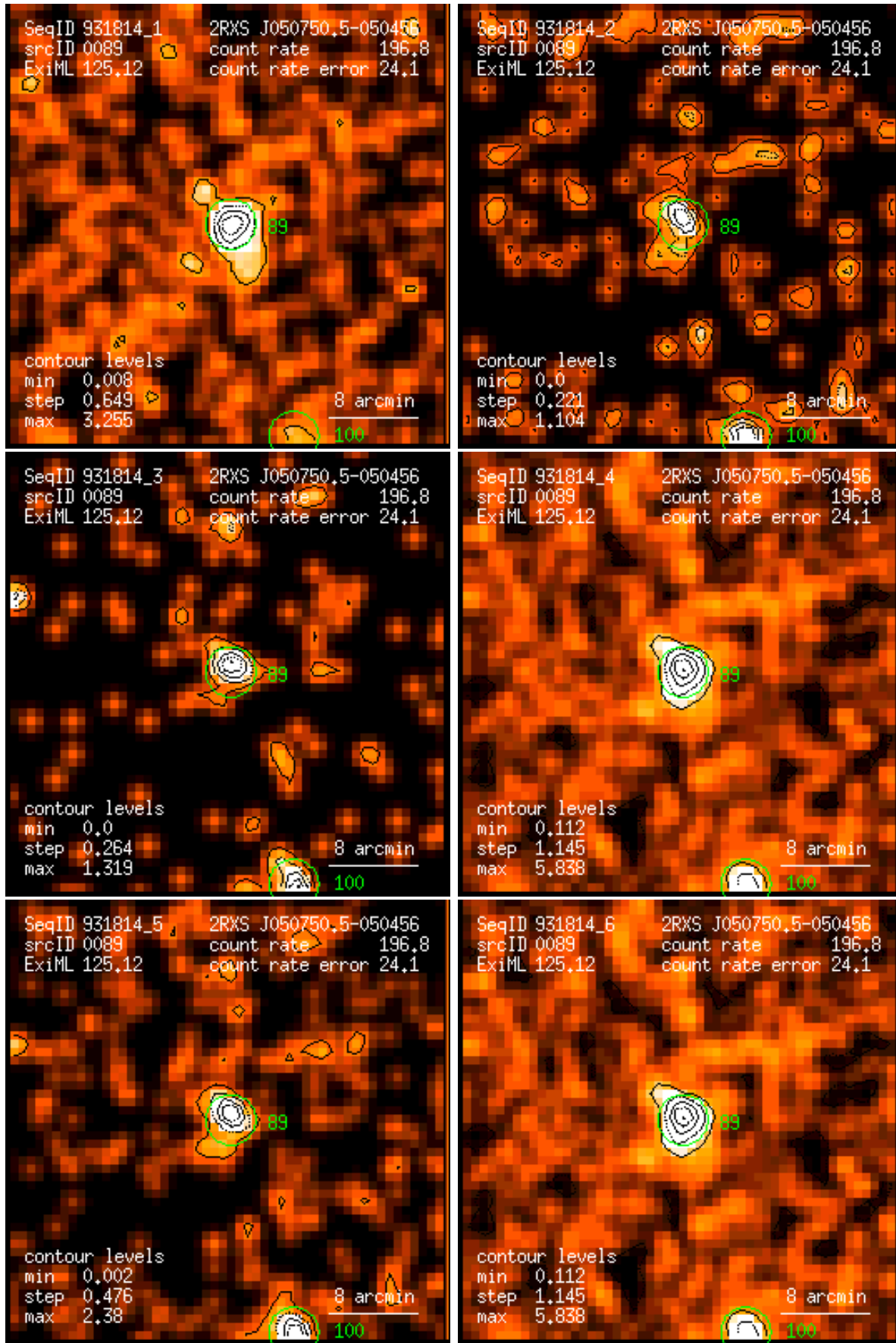
Figure 89: RASS 931814: detection 0089: band rate images, Gaussian filter: (1) PSPC channels 11 – 41, (2) 52 – 90, (3) 91 – 201, (4) 11 – 235, (5) 52 – 201, (6) 11 – 201. Broad band rates in counts/ks. Band rate contour levels in counts/ks/arcmin 2 .
