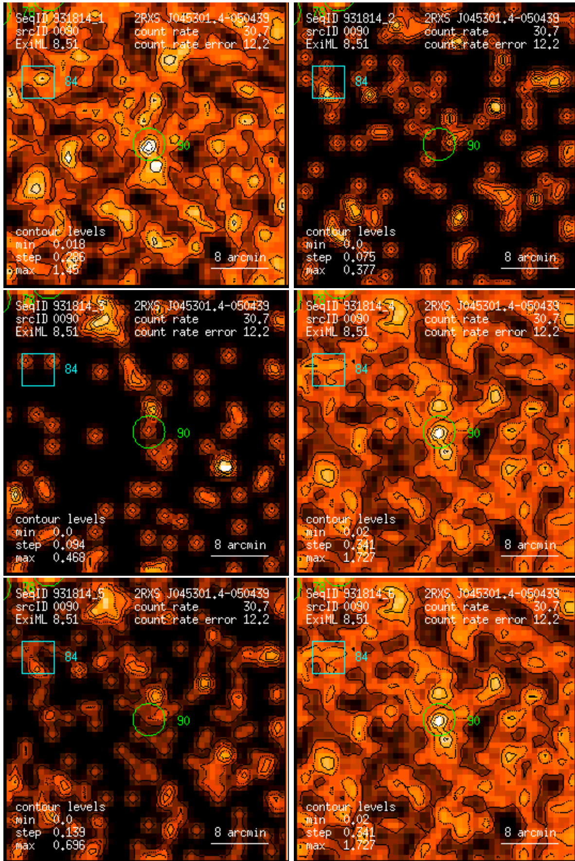
Figure 90: RASS 931814: detection 0090: band rate images, Gaussian filter: (1) PSPC channels 11 – 41, (2) 52 – 90, (3) 91 – 201, (4) 11 – 235, (5) 52 – 201, (6) 11 – 201. Broad band rates in counts/ks. Band rate contour levels in counts/ks/arcmin 2 .
