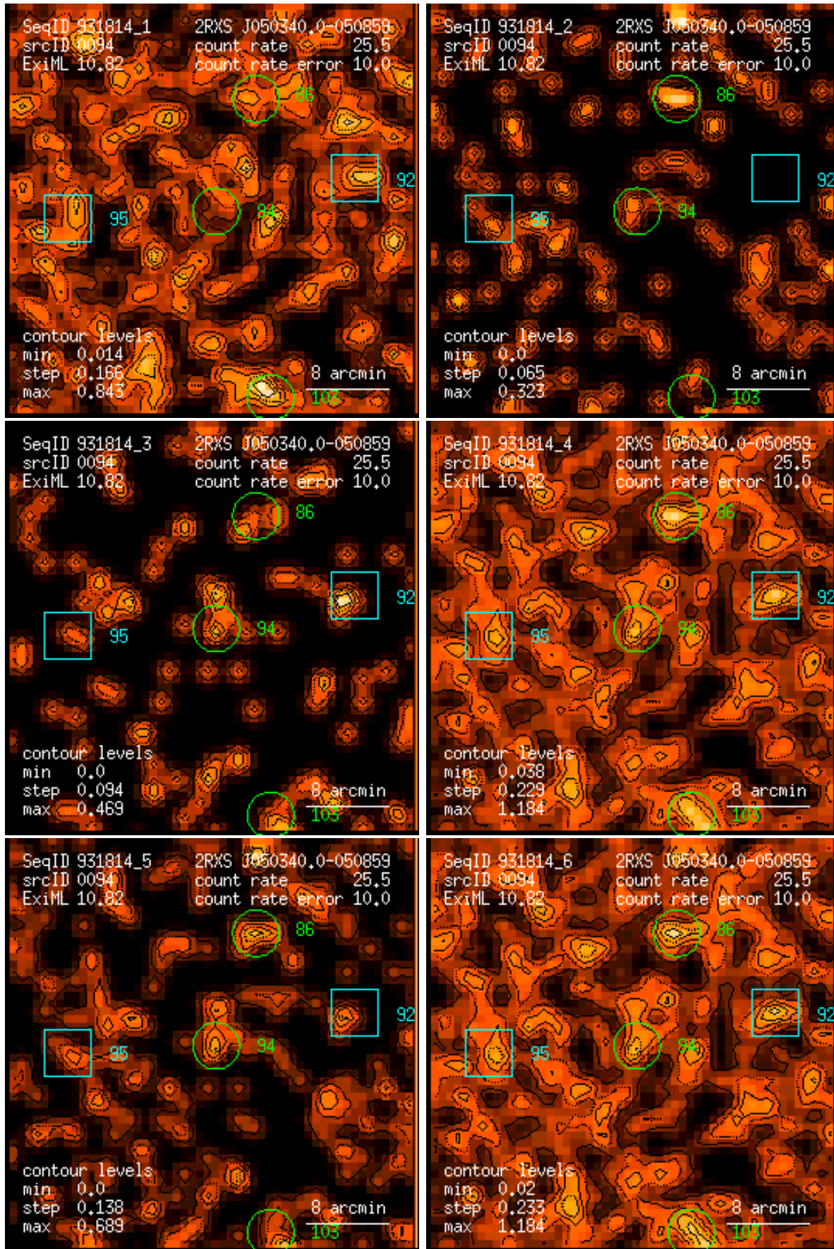
Figure 94: RASS 931814: detection 0094: band rate images, Gaussian filter: (1) PSPC channels 11 – 41, (2) 52 – 90, (3) 91 – 201, (4) 11 – 235, (5) 52 – 201, (6) 11 – 201. Broad band rates in counts/ks. Band rate contour levels in counts/ks/arcmin 2 .
