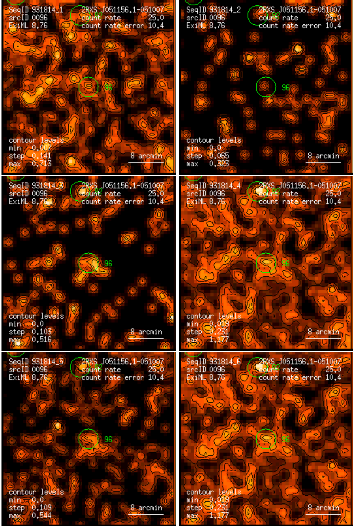
Figure 96: RASS 931814: detection 0096: band rate images, Gaussian filter: (1) PSPC channels 11 – 41, (2) 52 – 90, (3) 91 – 201, (4) 11 – 235, (5) 52 – 201, (6) 11 – 201. Broad band rates in counts/ks. Band rate contour levels in counts/ks/arcmin 2 .
