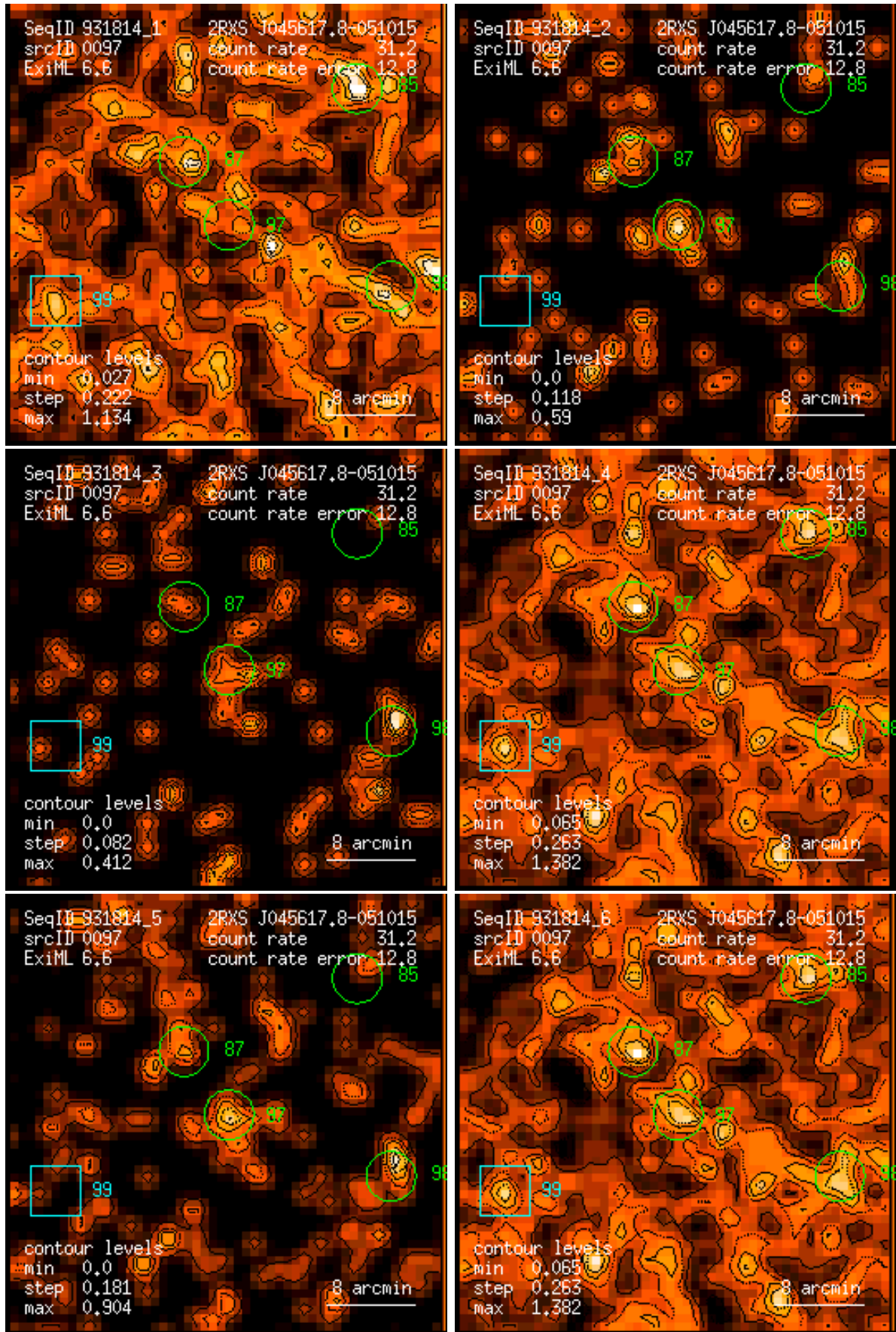
Figure 97: RASS 931814: detection 0097: band rate images, Gaussian filter: (1) PSPC channels 11 – 41, (2) 52 – 90, (3) 91 – 201, (4) 11 – 235, (5) 52 – 201, (6) 11 – 201. Broad band rates in counts/ks. Band rate contour levels in counts/ks/arcmin 2 .
