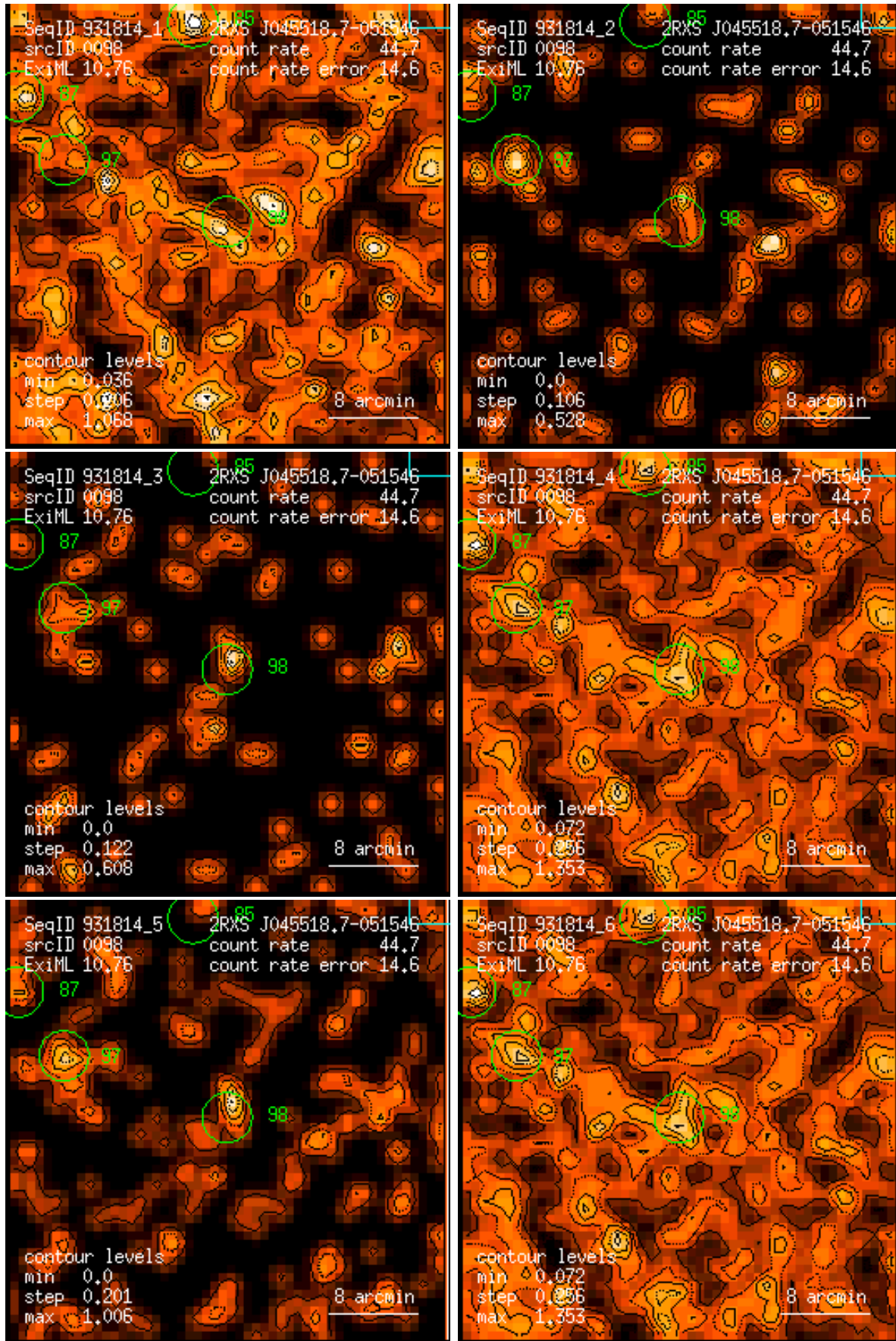
Figure 98: RASS 931814: detection 0098: band rate images, Gaussian filter: (1) PSPC channels 11 – 41, (2) 52 – 90, (3) 91 – 201, (4) 11 – 235, (5) 52 – 201, (6) 11 – 201. Broad band rates in counts/ks. Band rate contour levels in counts/ks/arcmin 2 .
