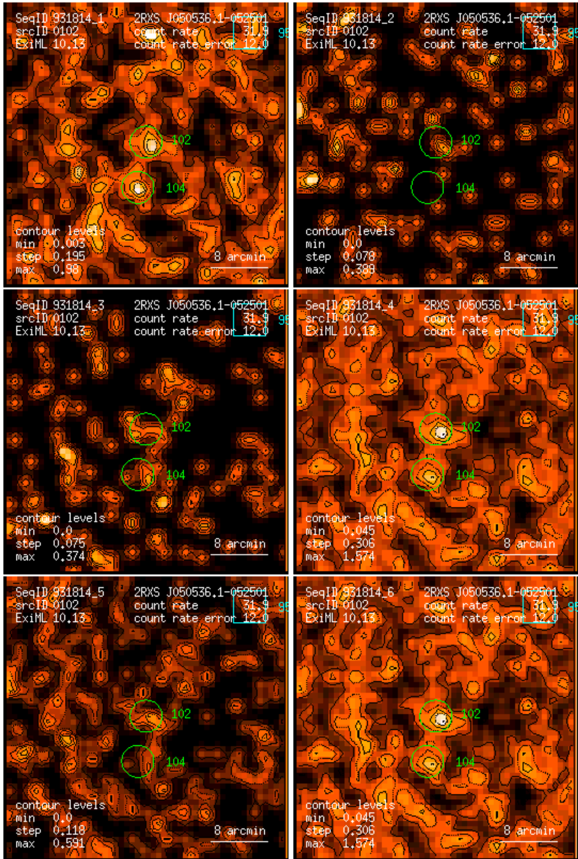
Figure 102: RASS 931814: detection 0102: band rate images, Gaussian filter: (1) PSPC channels 11 – 41, (2) 52 – 90, (3) 91 – 201, (4) 11 – 235, (5) 52 – 201, (6) 11 – 201. Broad band rates in counts/ks. Band rate contour levels in counts/ks/arcmin 2 .
