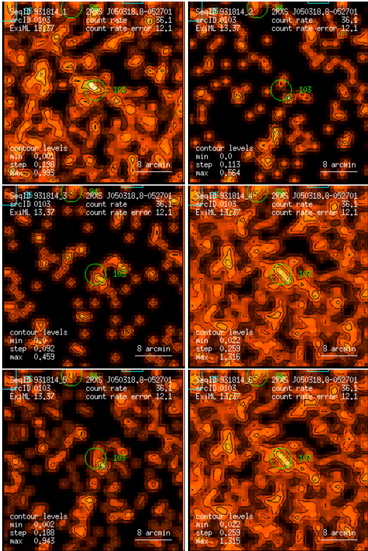
Figure 103: RASS 931814: detection 0103: band rate images, Gaussian filter: (1) PSPC channels 11 – 41, (2) 52 – 90, (3) 91 – 201, (4) 11 – 235, (5) 52 – 201, (6) 11 – 201. Broad band rates in counts/ks. Band rate contour levels in counts/ks/arcmin 2 .
