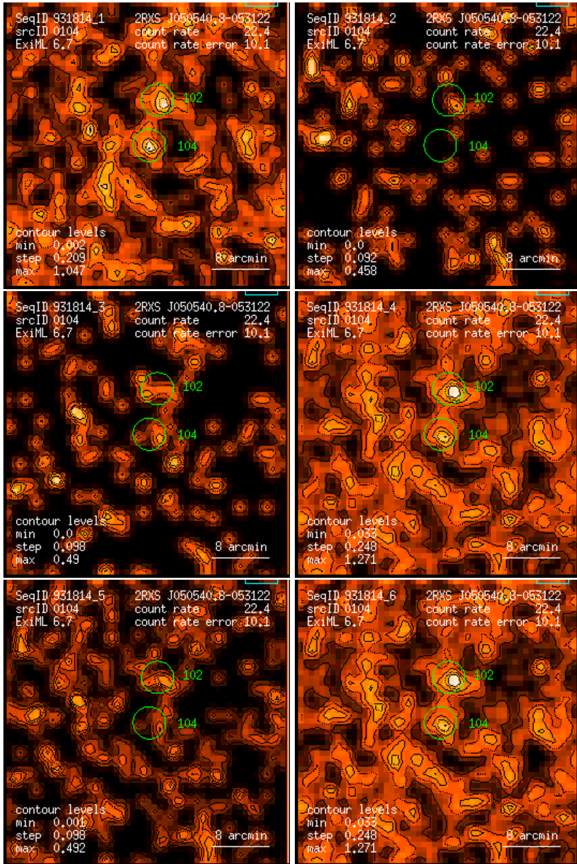
Figure 104: RASS 931814: detection 0104: band rate images, Gaussian filter: (1) PSPC channels 11 – 41, (2) 52 – 90, (3) 91 – 201, (4) 11 – 235, (5) 52 – 201, (6) 11 – 201. Broad band rates in counts/ks. Band rate contour levels in counts/ks/arcmin 2 .
