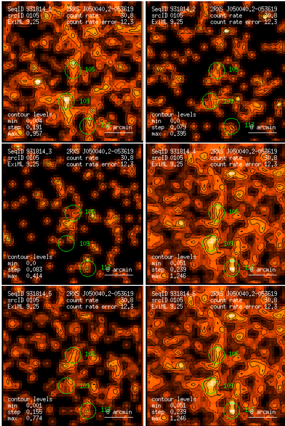
Figure 105: RASS 931814: detection 0105: band rate images, Gaussian filter: (1) PSPC channels 11 – 41, (2) 52 – 90, (3) 91 – 201, (4) 11 – 235, (5) 52 – 201, (6) 11 – 201. Broad band rates in counts/ks. Band rate contour levels in counts/ks/arcmin 2 .
