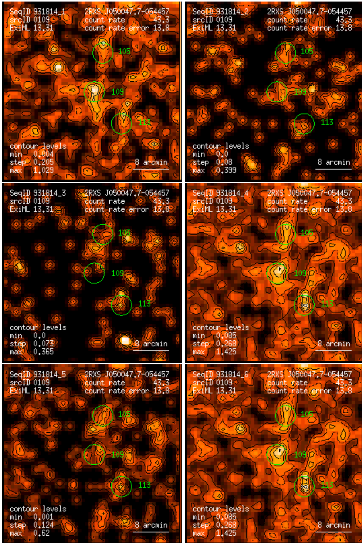
Figure 109: RASS 931814: detection 0109: band rate images, Gaussian filter: (1) PSPC channels 11 – 41, (2) 52 – 90, (3) 91 – 201, (4) 11 – 235, (5) 52 – 201, (6) 11 – 201. Broad band rates in counts/ks. Band rate contour levels in counts/ks/arcmin 2 .
