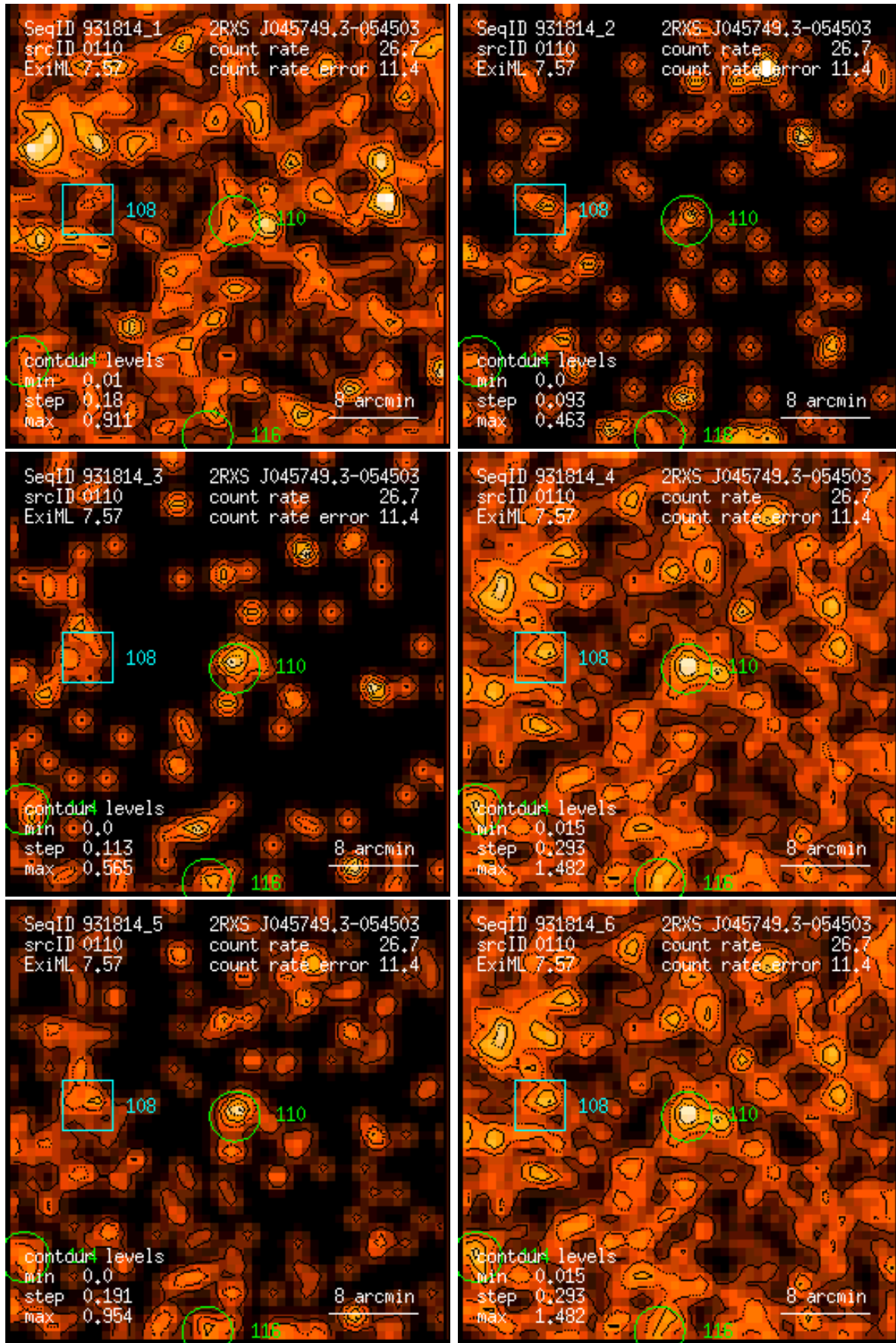
Figure 110: RASS 931814: detection 0110: band rate images, Gaussian filter: (1) PSPC channels 11 – 41, (2) 52 – 90, (3) 91 – 201, (4) 11 – 235, (5) 52 – 201, (6) 11 – 201. Broad band rates in counts/ks. Band rate contour levels in counts/ks/arcmin 2 .
