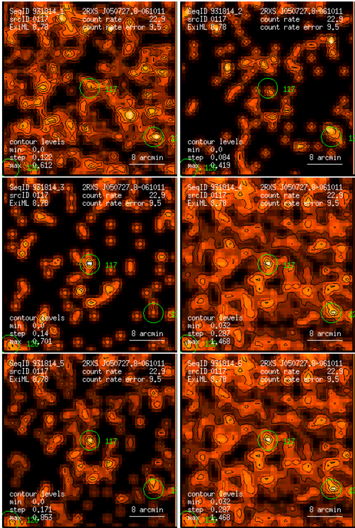
Figure 117: RASS 931814: detection 0117: band rate images, Gaussian filter: (1) PSPC channels 11 – 41, (2) 52 – 90, (3) 91 – 201, (4) 11 – 235, (5) 52 – 201, (6) 11 – 201. Broad band rates in counts/ks. Band rate contour levels in counts/ks/arcmin 2 .
