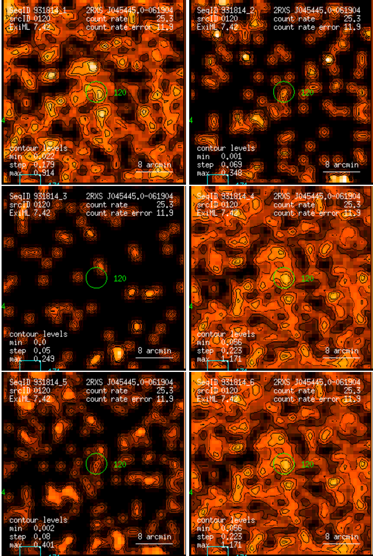
Figure 120: RASS 931814: detection 0120: band rate images, Gaussian filter: (1) PSPC channels 11 – 41, (2) 52 – 90, (3) 91 – 201, (4) 11 – 235, (5) 52 – 201, (6) 11 – 201. Broad band rates in counts/ks. Band rate contour levels in counts/ks/arcmin 2 .
