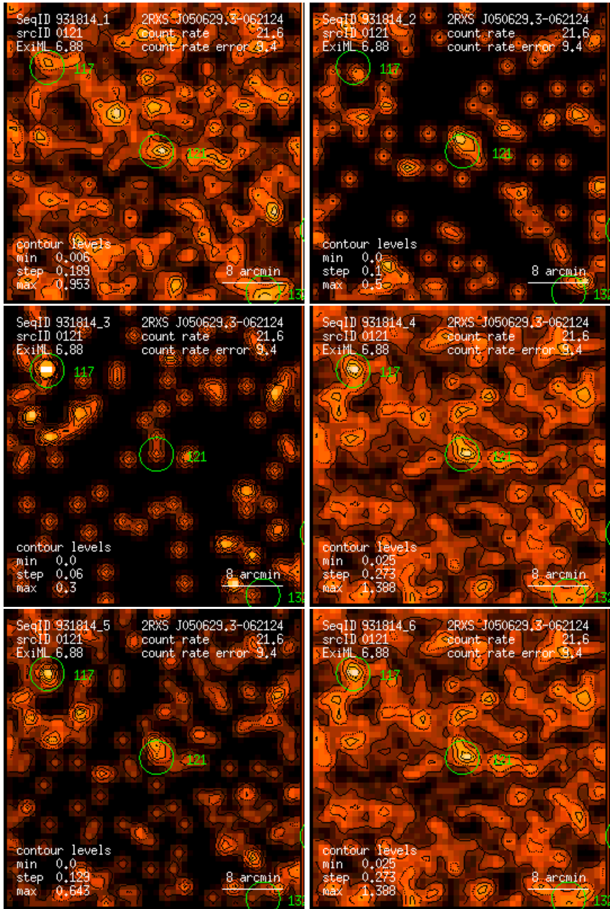
Figure 121: RASS 931814: detection 0121: band rate images, Gaussian filter: (1) PSPC channels 11 – 41, (2) 52 – 90, (3) 91 – 201, (4) 11 – 235, (5) 52 – 201, (6) 11 – 201. Broad band rates in counts/ks. Band rate contour levels in counts/ks/arcmin 2 .
