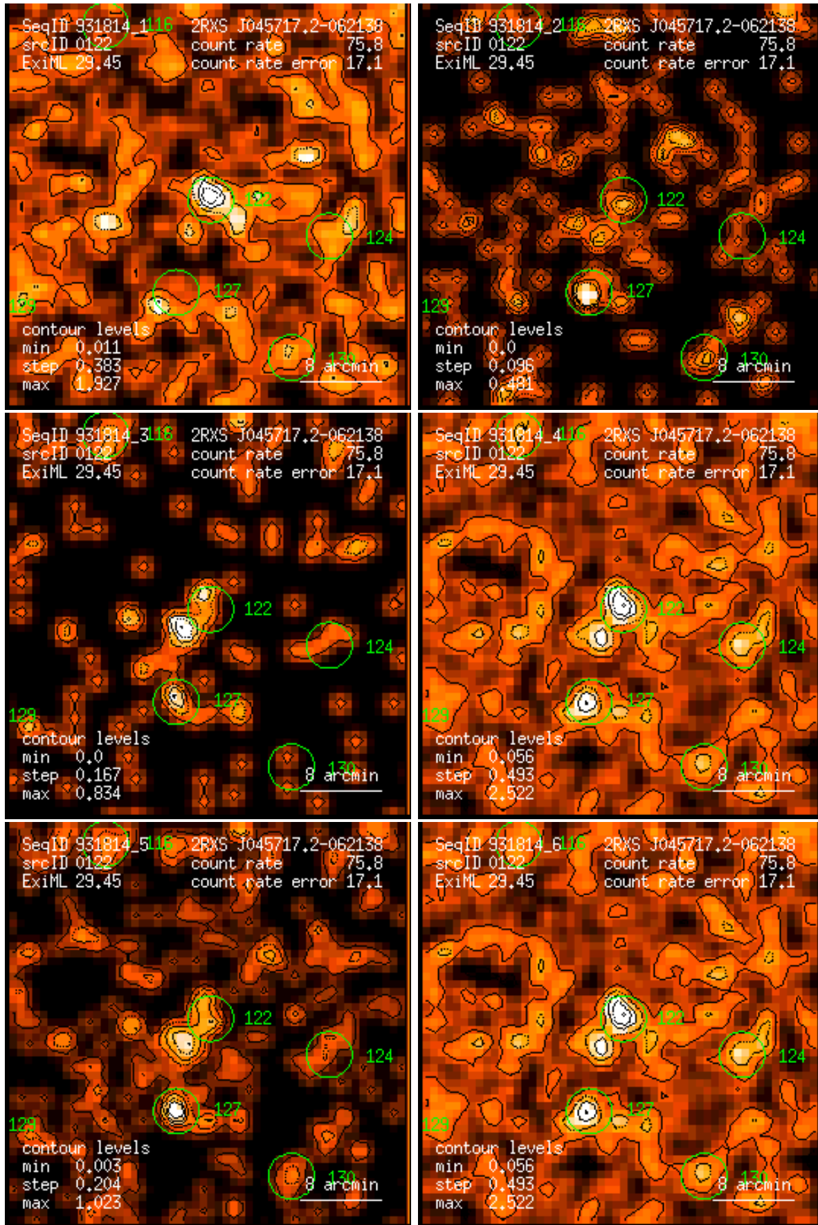
Figure 122: RASS 931814: detection 0122: band rate images, Gaussian filter: (1) PSPC channels 11 – 41, (2) 52 – 90, (3) 91 – 201, (4) 11 – 235, (5) 52 – 201, (6) 11 – 201. Broad band rates in counts/ks. Band rate contour levels in counts/ks/arcmin 2 .
