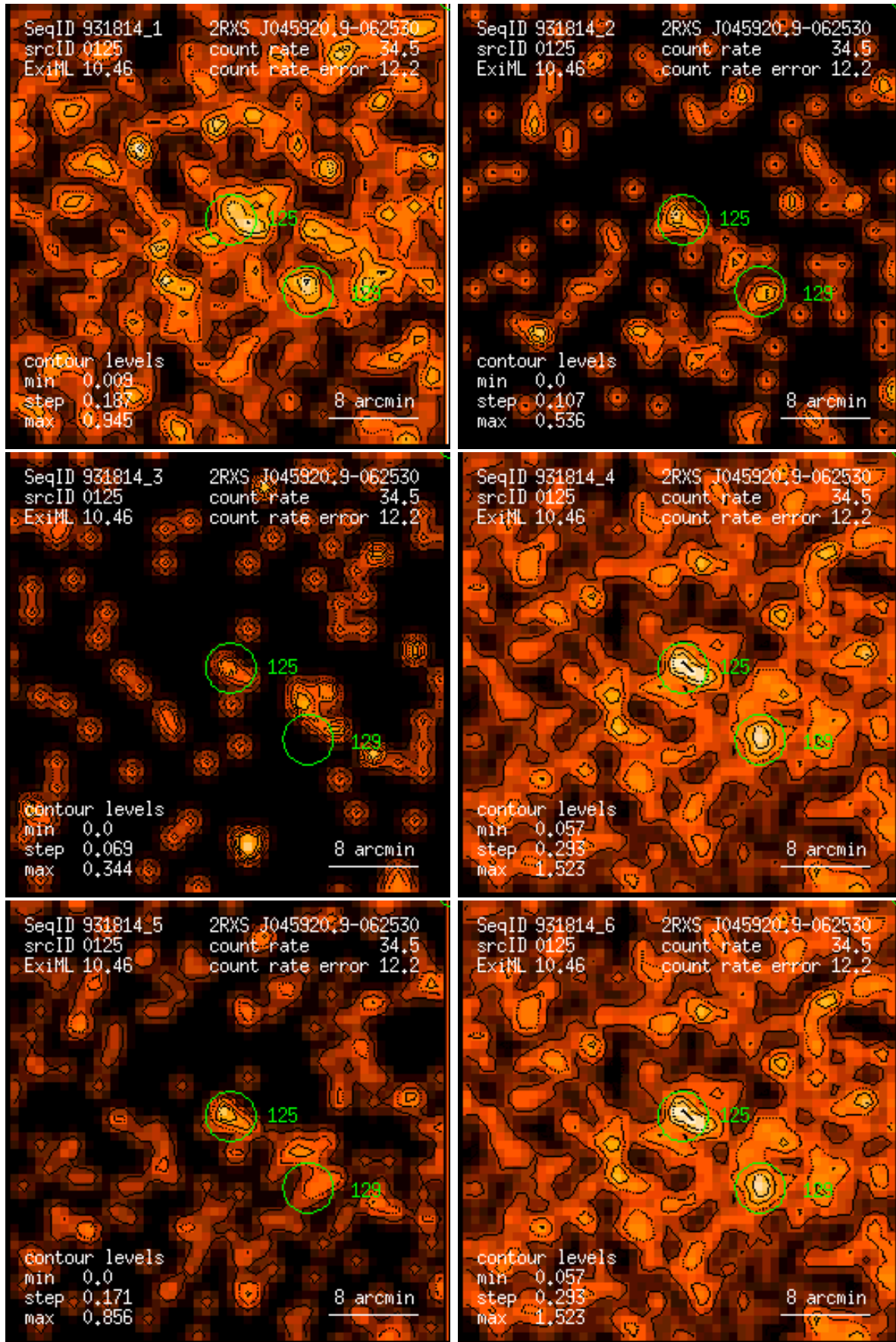
Figure 125: RASS 931814: detection 0125: band rate images, Gaussian filter: (1) PSPC channels 11 – 41, (2) 52 – 90, (3) 91 – 201, (4) 11 – 235, (5) 52 – 201, (6) 11 – 201. Broad band rates in counts/ks. Band rate contour levels in counts/ks/arcmin 2 .
