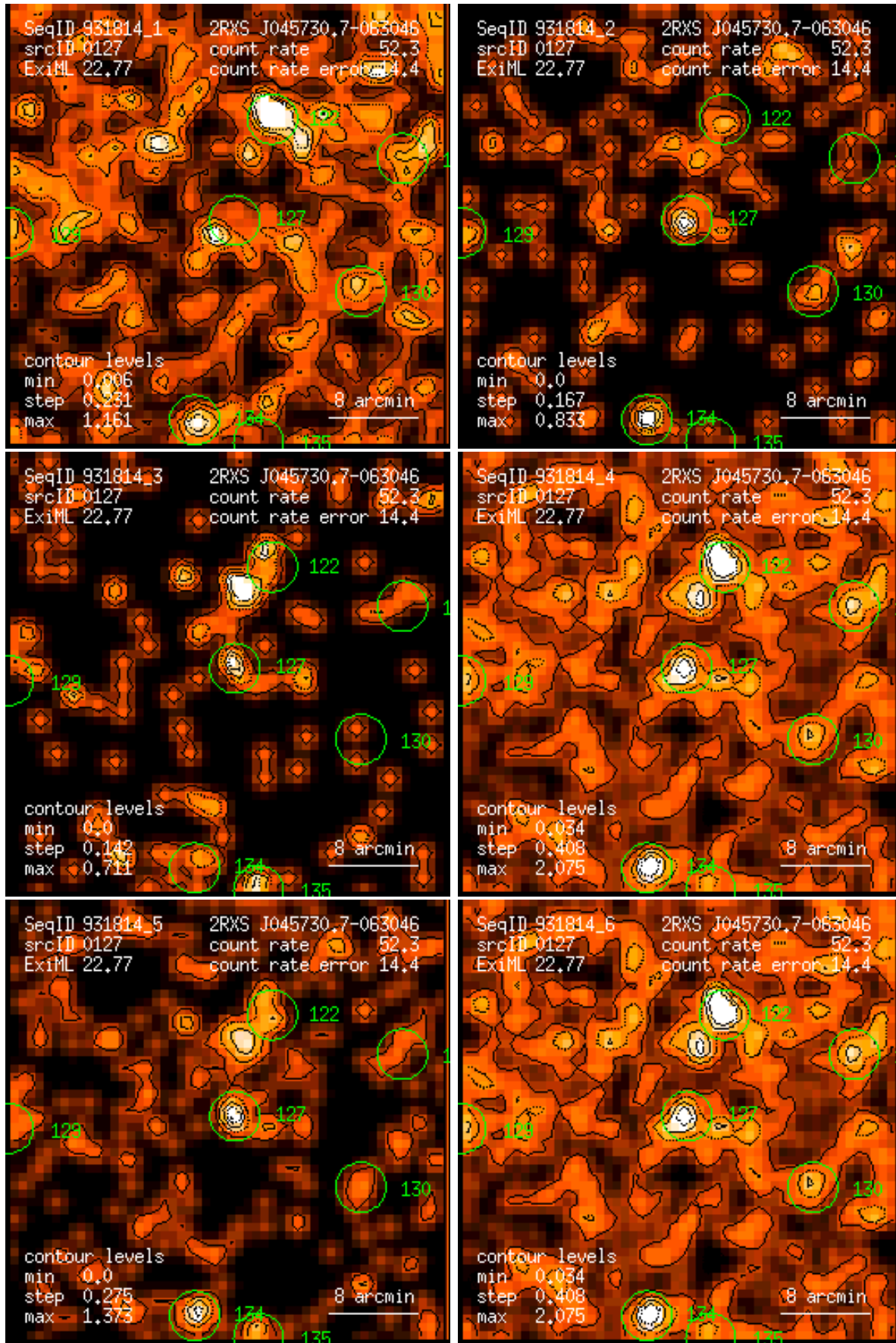
Figure 127: RASS 931814: detection 0127: band rate images, Gaussian filter: (1) PSPC channels 11 – 41, (2) 52 – 90, (3) 91 – 201, (4) 11 – 235, (5) 52 – 201, (6) 11 – 201. Broad band rates in counts/ks. Band rate contour levels in counts/ks/arcmin 2 .
