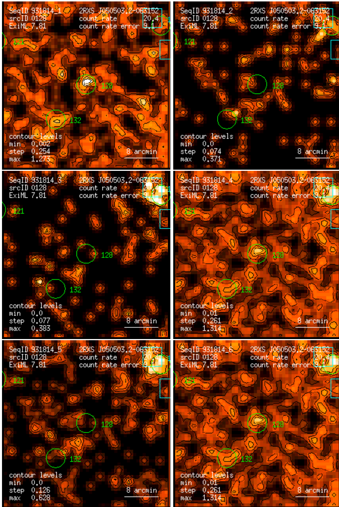
Figure 128: RASS 931814: detection 0128: band rate images, Gaussian filter: (1) PSPC channels 11 – 41, (2) 52 – 90, (3) 91 – 201, (4) 11 – 235, (5) 52 – 201, (6) 11 – 201. Broad band rates in counts/ks. Band rate contour levels in counts/ks/arcmin 2 .
