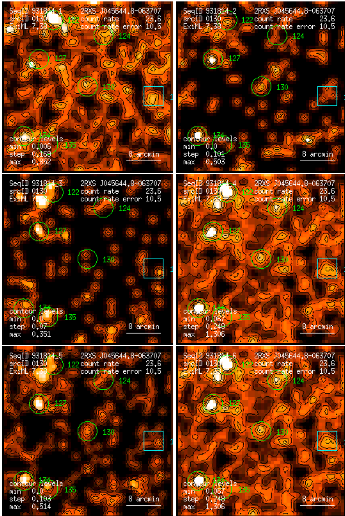
Figure 130: RASS 931814: detection 0130: band rate images, Gaussian filter: (1) PSPC channels 11 – 41, (2) 52 – 90, (3) 91 – 201, (4) 11 – 235, (5) 52 – 201, (6) 11 – 201. Broad band rates in counts/ks. Band rate contour levels in counts/ks/arcmin 2 .
