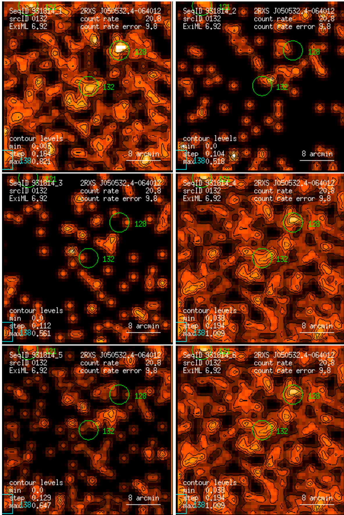
Figure 132: RASS 931814: detection 0132: band rate images, Gaussian filter: (1) PSPC channels 11 – 41, (2) 52 – 90, (3) 91 – 201, (4) 11 – 235, (5) 52 – 201, (6) 11 – 201. Broad band rates in counts/ks. Band rate contour levels in counts/ks/arcmin 2 .
