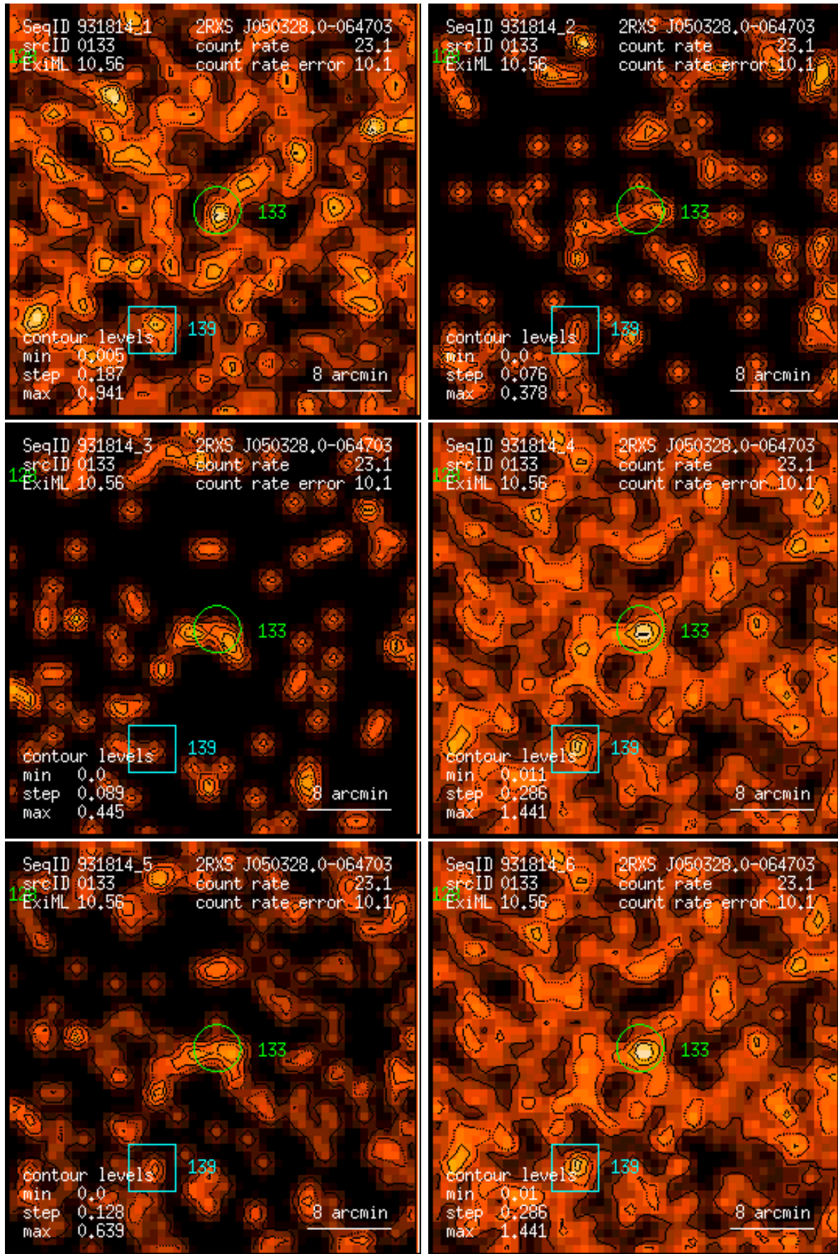
Figure 133: RASS 931814: detection 0133: band rate images, Gaussian filter: (1) PSPC channels 11 – 41, (2) 52 – 90, (3) 91 – 201, (4) 11 – 235, (5) 52 – 201, (6) 11 – 201. Broad band rates in counts/ks. Band rate contour levels in counts/ks/arcmin 2 .
