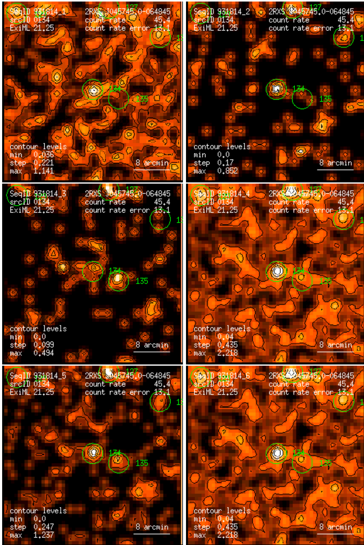
Figure 134: RASS 931814: detection 0134: band rate images, Gaussian filter: (1) PSPC channels 11 – 41, (2) 52 – 90, (3) 91 – 201, (4) 11 – 235, (5) 52 – 201, (6) 11 – 201. Broad band rates in counts/ks. Band rate contour levels in counts/ks/arcmin 2 .
