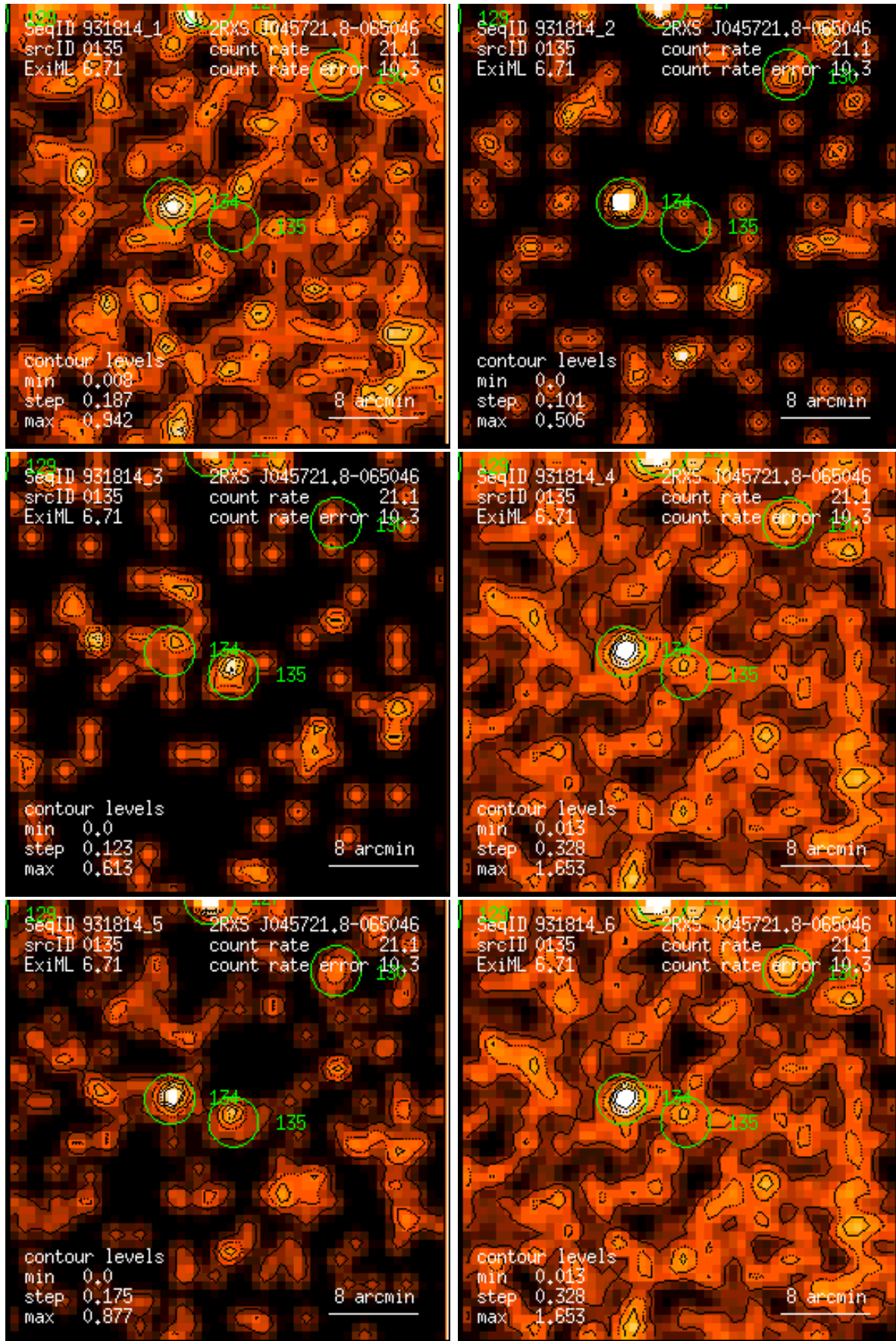
Figure 135: RASS 931814: detection 0135: band rate images, Gaussian filter: (1) PSPC channels 11 – 41, (2) 52 – 90, (3) 91 – 201, (4) 11 – 235, (5) 52 – 201, (6) 11 – 201. Broad band rates in counts/ks. Band rate contour levels in counts/ks/arcmin 2 .
