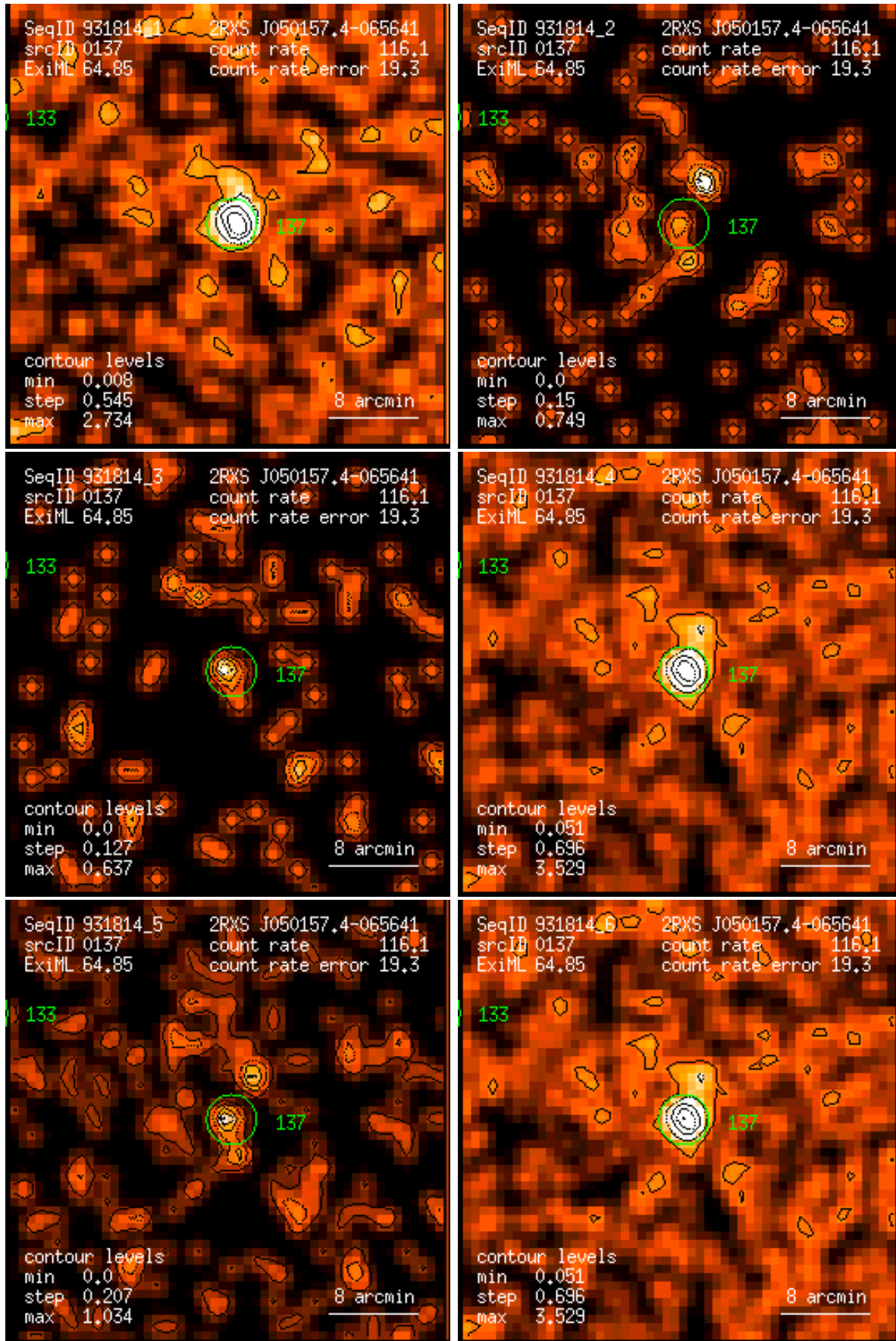
Figure 137: RASS 931814: detection 0137: band rate images, Gaussian filter: (1) PSPC channels 11 – 41, (2) 52 – 90, (3) 91 – 201, (4) 11 – 235, (5) 52 – 201, (6) 11 – 201. Broad band rates in counts/ks. Band rate contour levels in counts/ks/arcmin 2 .
