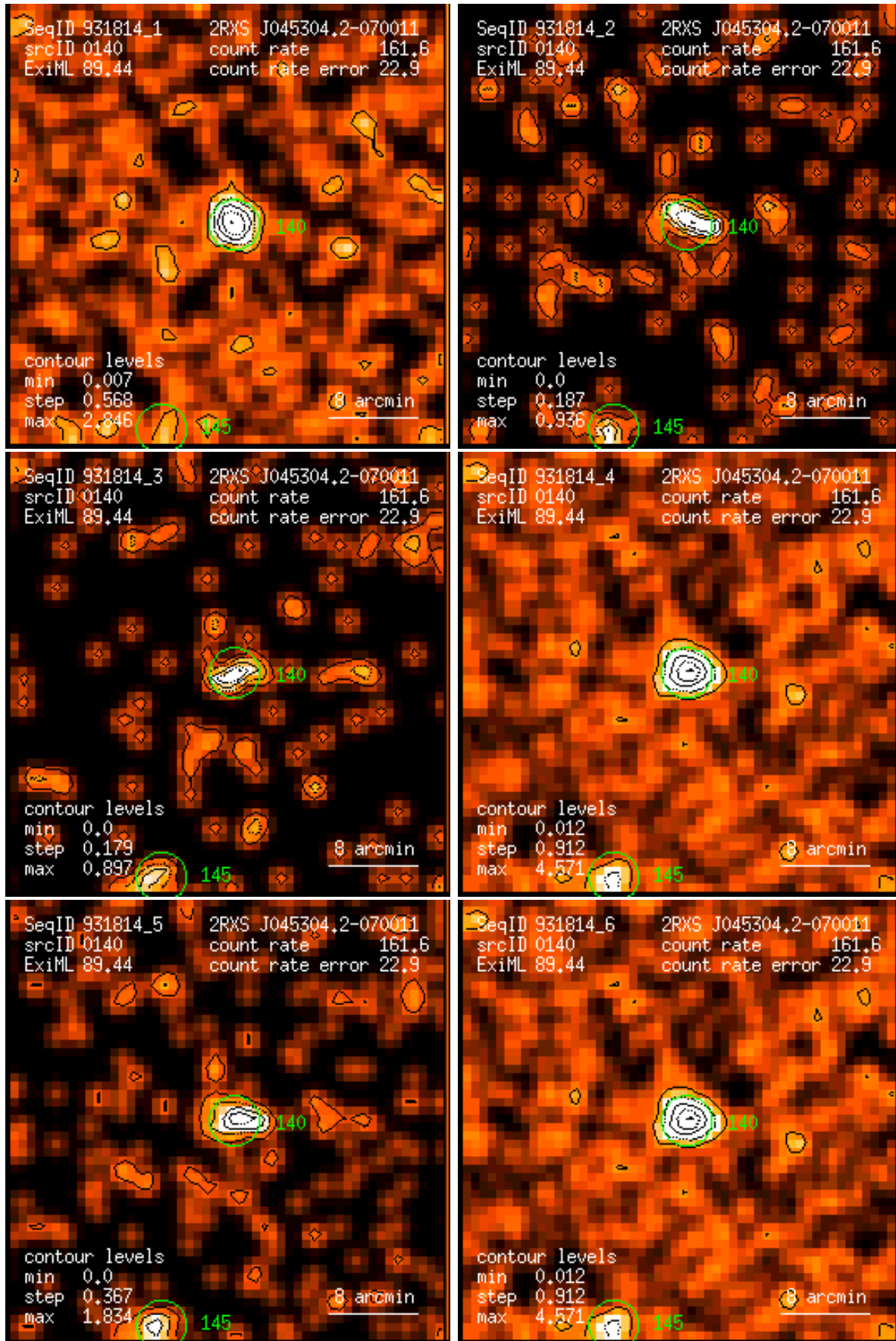
Figure 140: RASS 931814: detection 0140: band rate images, Gaussian filter: (1) PSPC channels 11 – 41, (2) 52 – 90, (3) 91 – 201, (4) 11 – 235, (5) 52 – 201, (6) 11 – 201. Broad band rates in counts/ks. Band rate contour levels in counts/ks/arcmin 2 .
