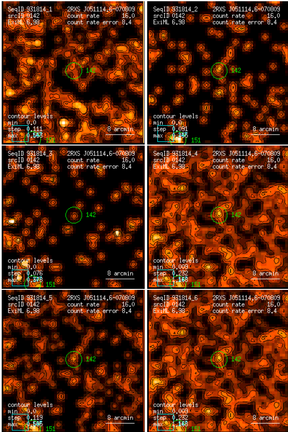
Figure 142: RASS 931814: detection 0142: band rate images, Gaussian filter: (1) PSPC channels 11 – 41, (2) 52 – 90, (3) 91 – 201, (4) 11 – 235, (5) 52 – 201, (6) 11 – 201. Broad band rates in counts/ks. Band rate contour levels in counts/ks/arcmin 2 .
