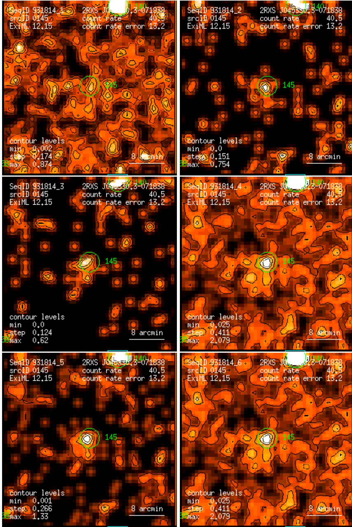
Figure 145: RASS 931814: detection 0145: band rate images, Gaussian filter: (1) PSPC channels 11 – 41, (2) 52 – 90, (3) 91 – 201, (4) 11 – 235, (5) 52 – 201, (6) 11 – 201. Broad band rates in counts/ks. Band rate contour levels in counts/ks/arcmin 2 .
