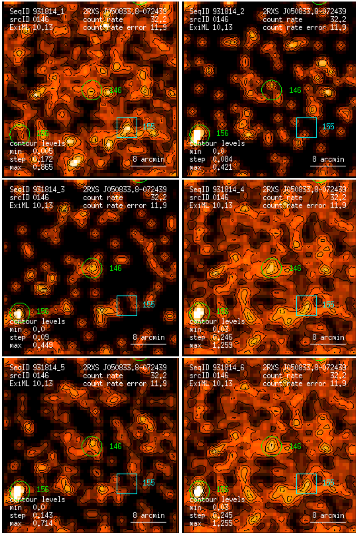
Figure 146: RASS 931814: detection 0146: band rate images, Gaussian filter: (1) PSPC channels 11 – 41, (2) 52 – 90, (3) 91 – 201, (4) 11 – 235, (5) 52 – 201, (6) 11 – 201. Broad band rates in counts/ks. Band rate contour levels in counts/ks/arcmin 2 .
