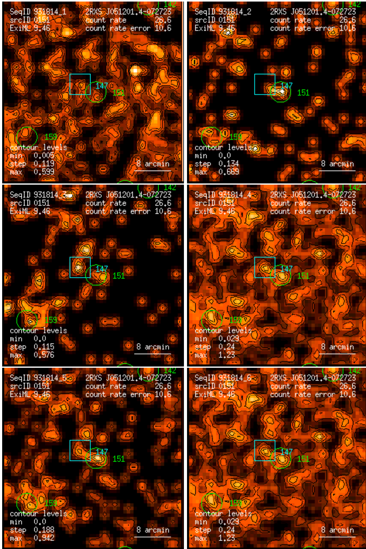
Figure 151: RASS 931814: detection 0151: band rate images, Gaussian filter: (1) PSPC channels 11 – 41, (2) 52 – 90, (3) 91 – 201, (4) 11 – 235, (5) 52 – 201, (6) 11 – 201. Broad band rates in counts/ks. Band rate contour levels in counts/ks/arcmin 2 .
