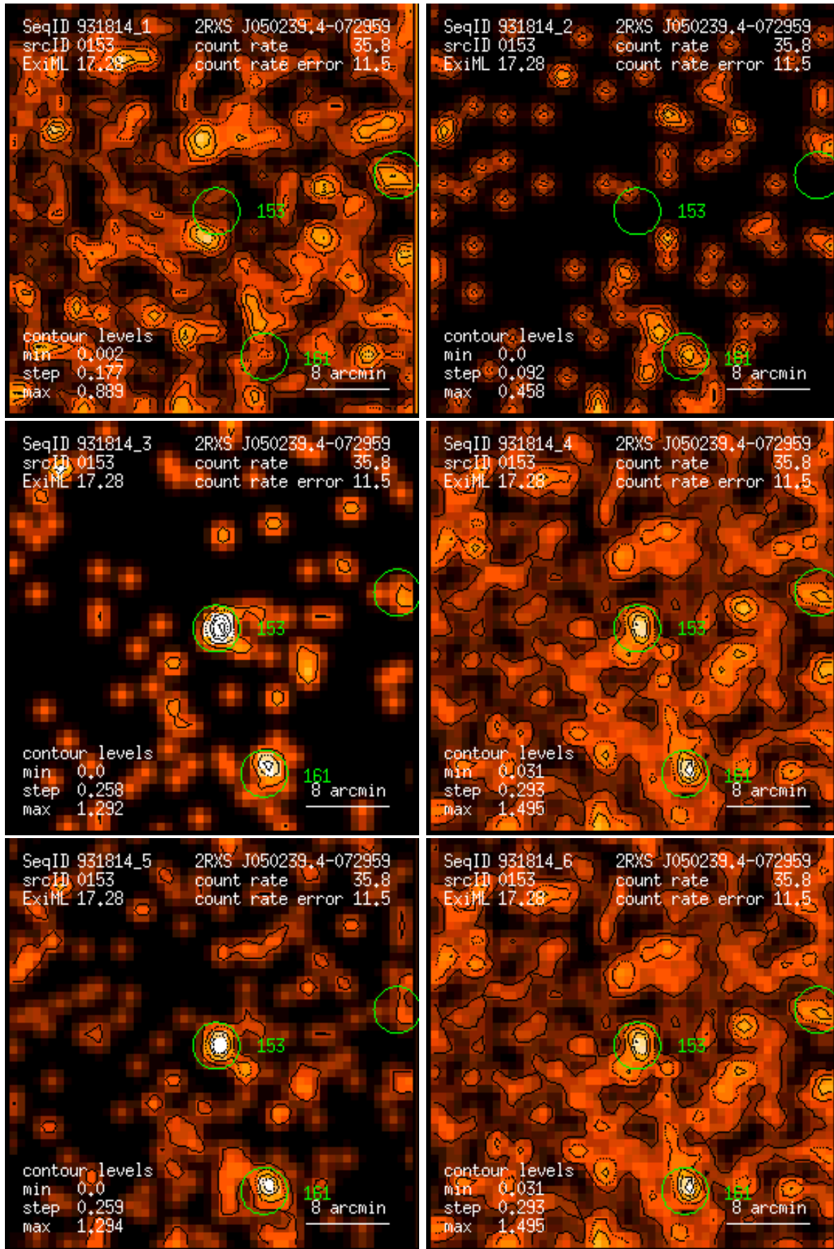
Figure 153: RASS 931814: detection 0153: band rate images, Gaussian filter: (1) PSPC channels 11 – 41, (2) 52 – 90, (3) 91 – 201, (4) 11 – 235, (5) 52 – 201, (6) 11 – 201. Broad band rates in counts/ks. Band rate contour levels in counts/ks/arcmin 2 .
