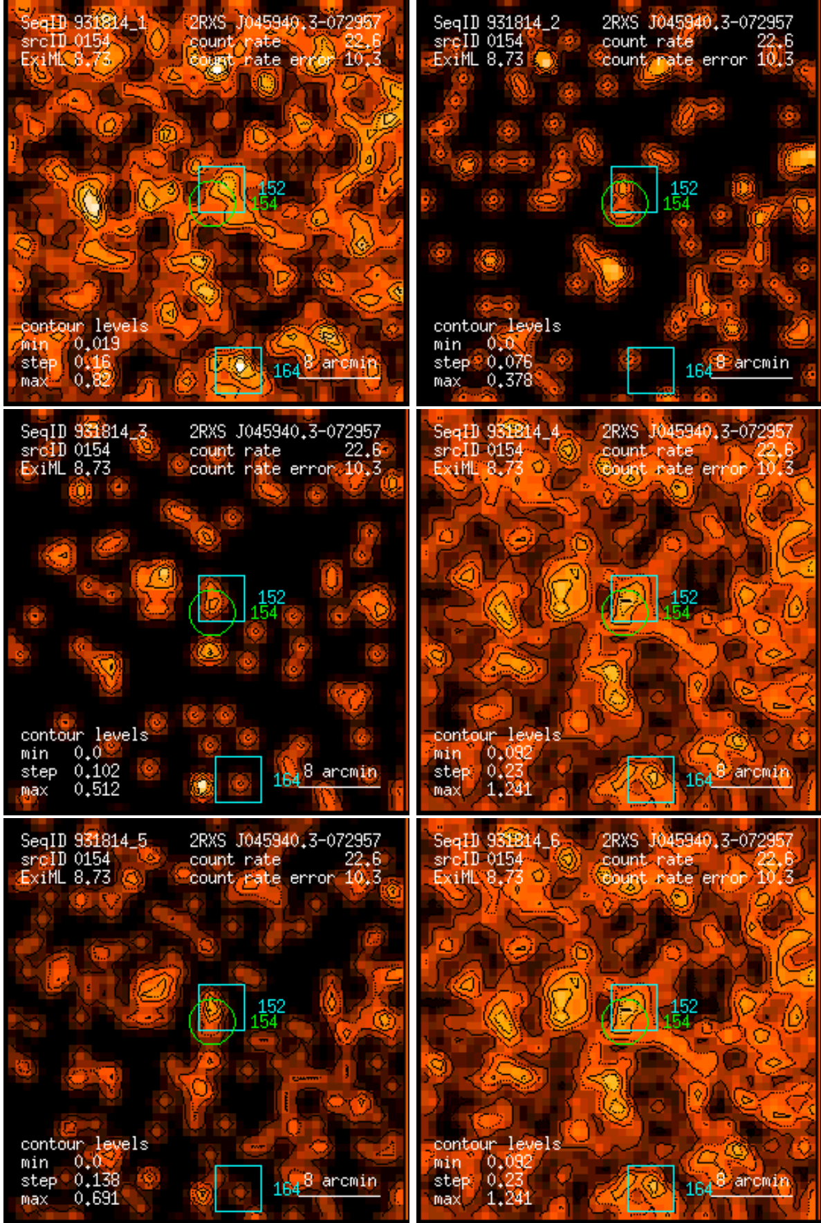
Figure 154: RASS 931814: detection 0154: band rate images, Gaussian filter: (1) PSPC channels 11 – 41, (2) 52 – 90, (3) 91 – 201, (4) 11 – 235, (5) 52 – 201, (6) 11 – 201. Broad band rates in counts/ks. Band rate contour levels in counts/ks/arcmin 2 .
