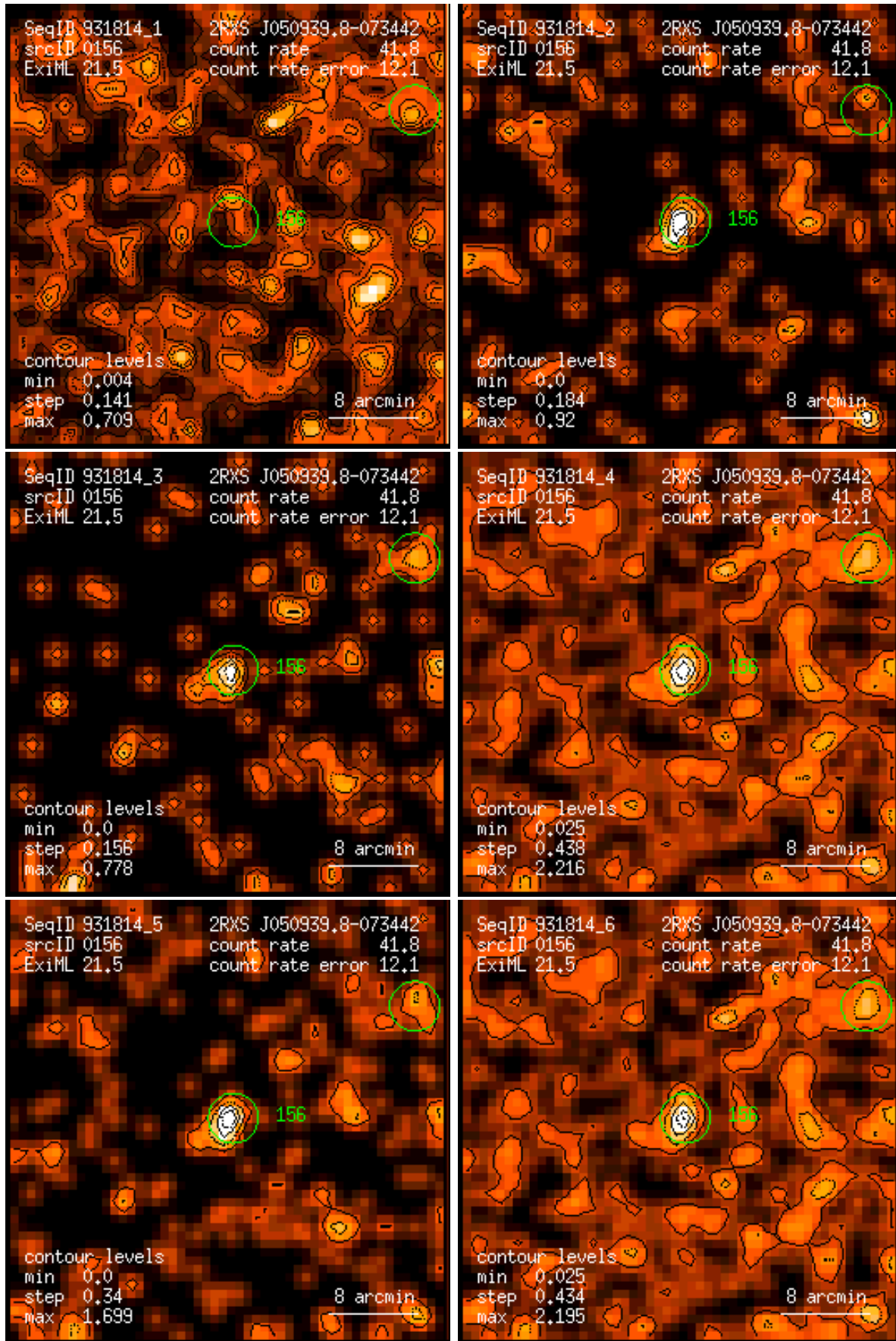
Figure 156: RASS 931814: detection 0156: band rate images, Gaussian filter: (1) PSPC channels 11 – 41, (2) 52 – 90, (3) 91 – 201, (4) 11 – 235, (5) 52 – 201, (6) 11 – 201. Broad band rates in counts/ks. Band rate contour levels in counts/ks/arcmin 2 .
