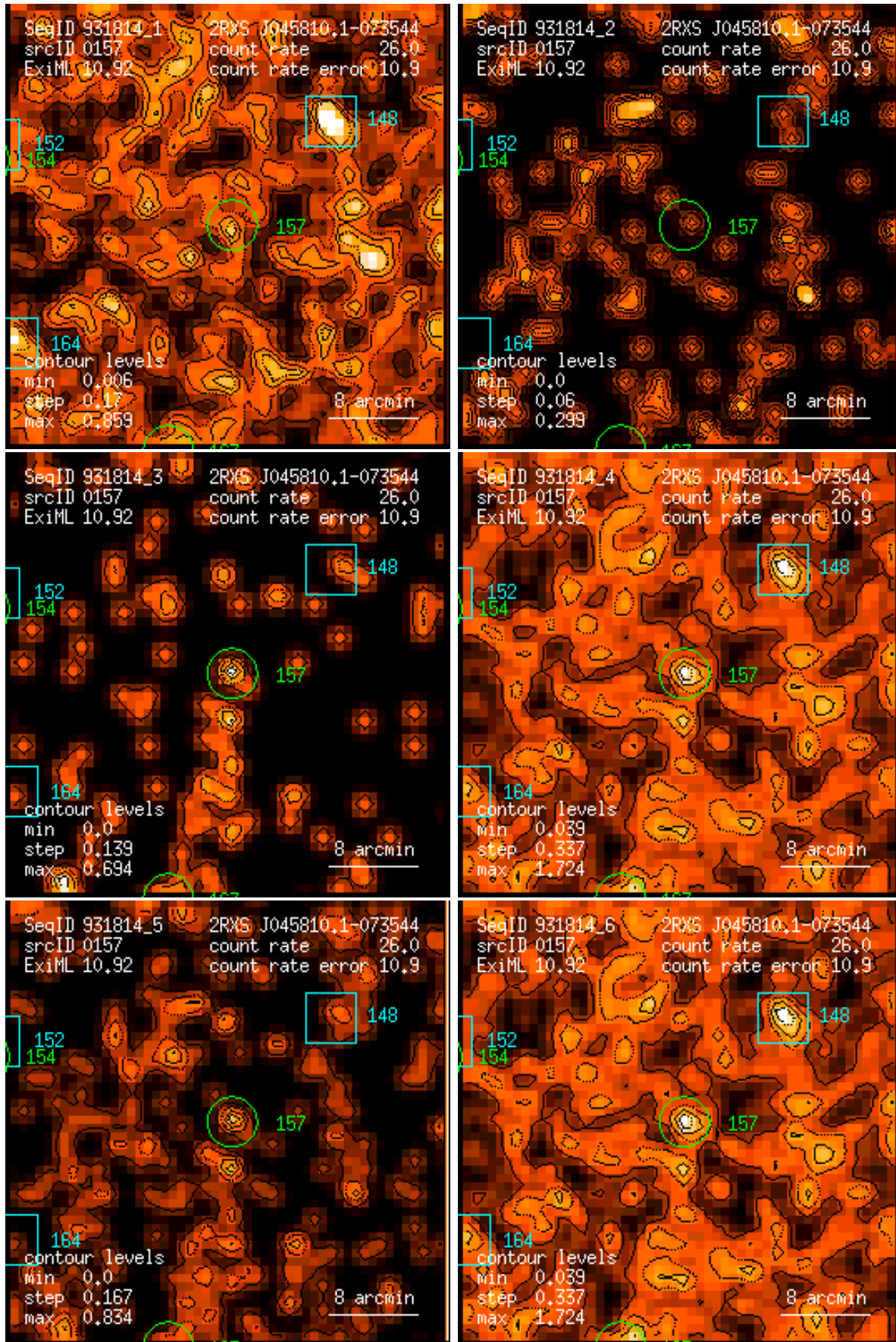
Figure 157: RASS 931814: detection 0157: band rate images, Gaussian filter: (1) PSPC channels 11 – 41, (2) 52 – 90, (3) 91 – 201, (4) 11 – 235, (5) 52 – 201, (6) 11 – 201. Broad band rates in counts/ks. Band rate contour levels in counts/ks/arcmin 2 .
