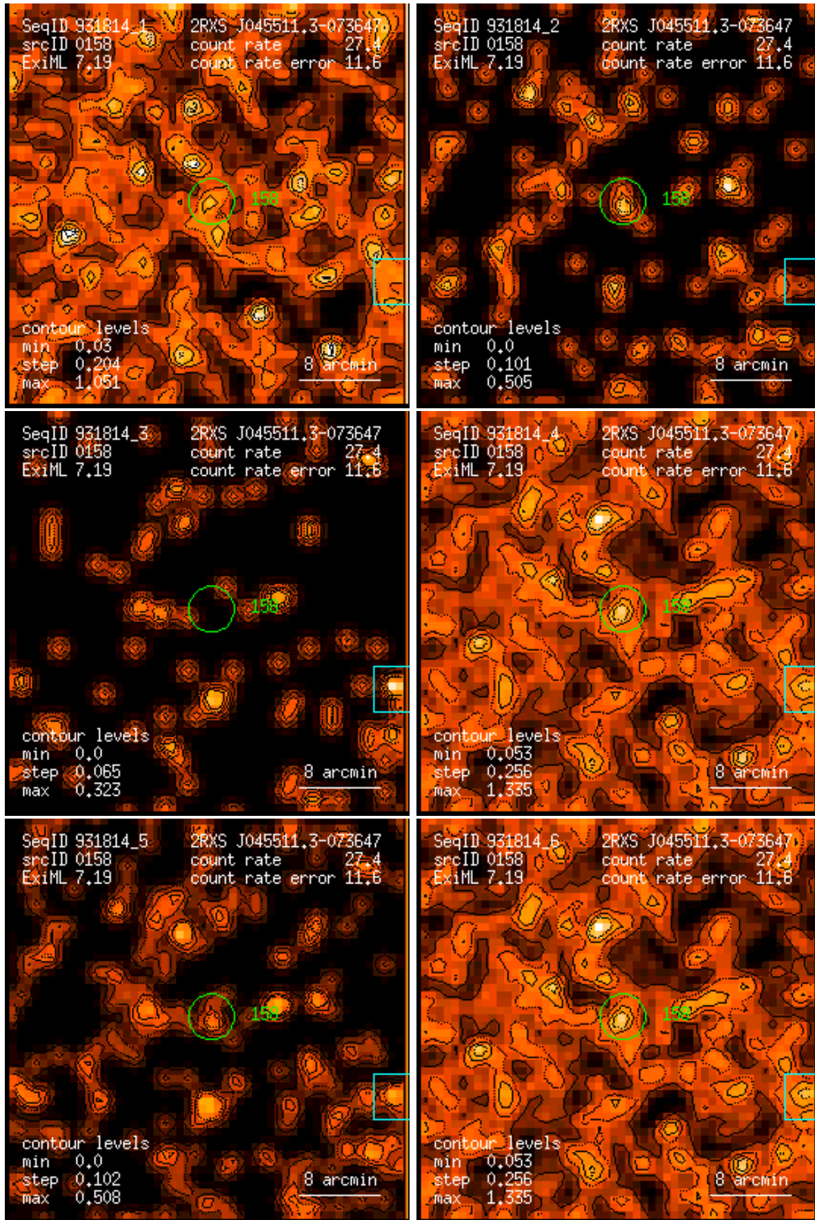
Figure 158: RASS 931814: detection 0158: band rate images, Gaussian filter: (1) PSPC channels 11 – 41, (2) 52 – 90, (3) 91 – 201, (4) 11 – 235, (5) 52 – 201, (6) 11 – 201. Broad band rates in counts/ks. Band rate contour levels in counts/ks/arcmin 2 .
