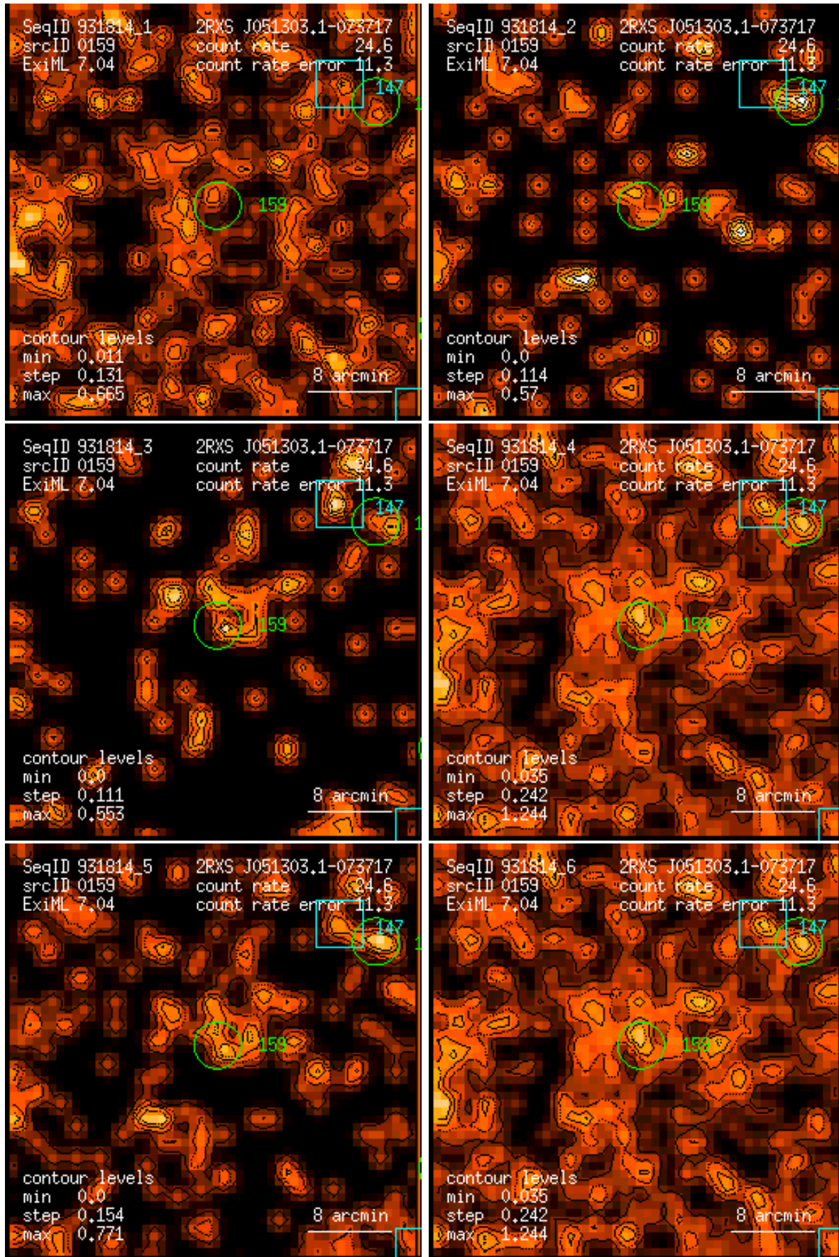
Figure 159: RASS 931814: detection 0159: band rate images, Gaussian filter: (1) PSPC channels 11 – 41, (2) 52 – 90, (3) 91 – 201, (4) 11 – 235, (5) 52 – 201, (6) 11 – 201. Broad band rates in counts/ks. Band rate contour levels in counts/ks/arcmin 2 .
